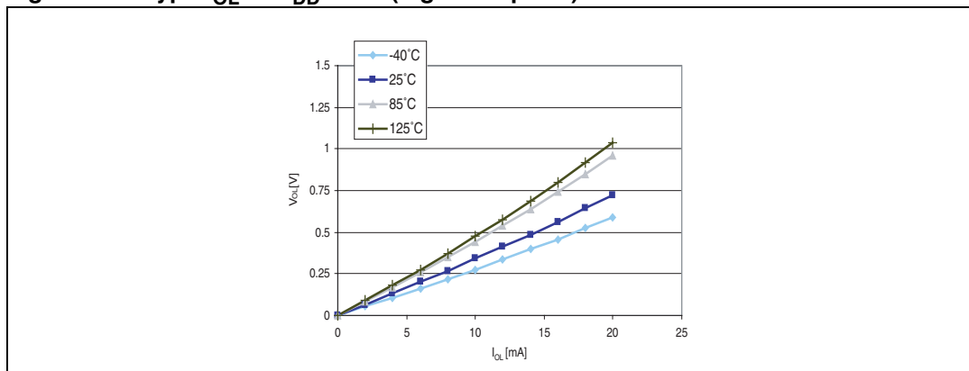
Figure 29. Typ. V_{OL} @ V_{DD} = 5\text{ V} (high sink ports)
