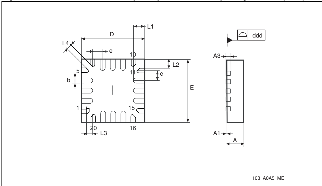
Figure 47. 20-lead, ultra thin, fine pitch quad flat no-lead package outline (3 x 3)
