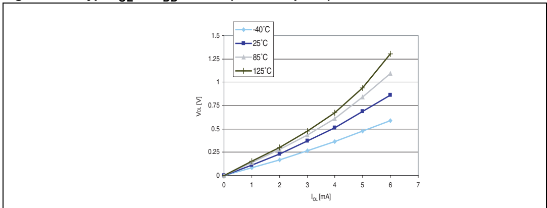
Figure 27. Typ. V_{OL} @ V_{DD} = 5\text{ V} (true open drain ports)
