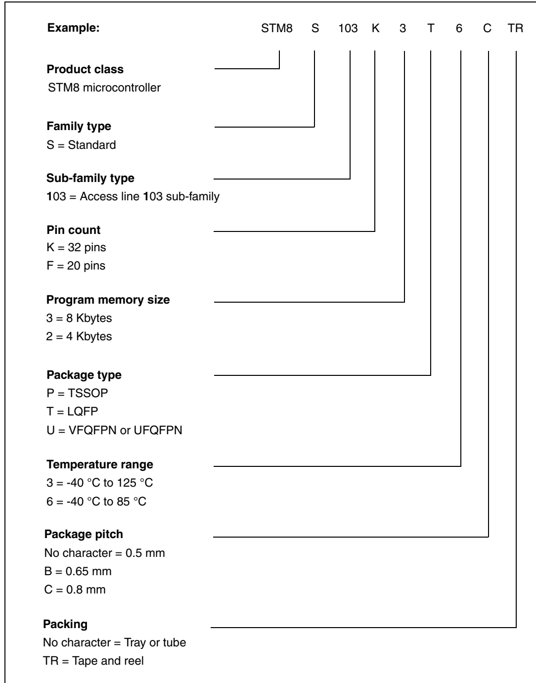
Figure 50. STM8S103x access line ordering information scheme
