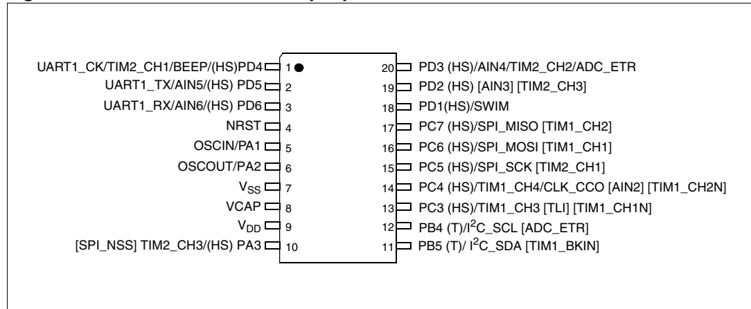
Figure 4. STM8S103F TSSOP20-pin pinout
