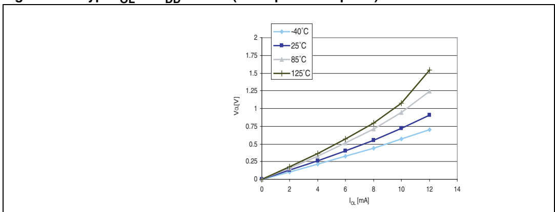
Figure 28. Typ. V_{OL} @ V_{DD} = 3.3\text{ V} (true open drain ports)
