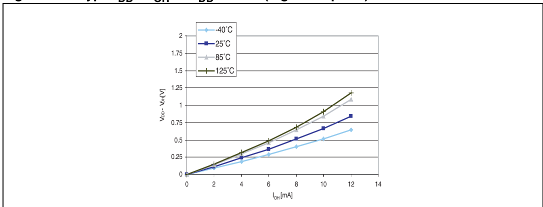
Figure 34. Typ. V_{DD} - V_{OH} @ V_{DD} = 3.3\text{ V} (high sink ports)
