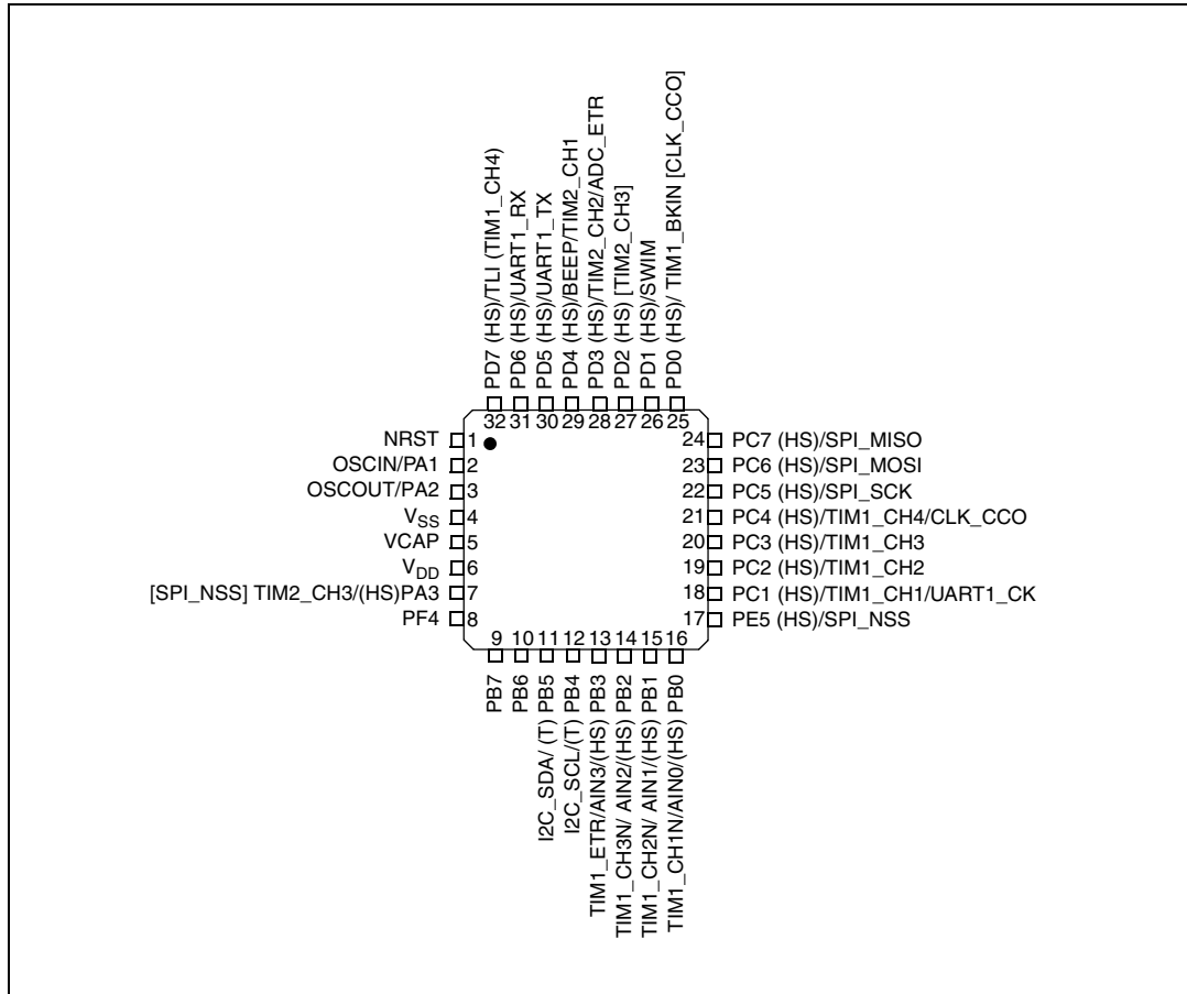
Figure 3. STM8S103K VFQFPN32/LQFP32 pinout
