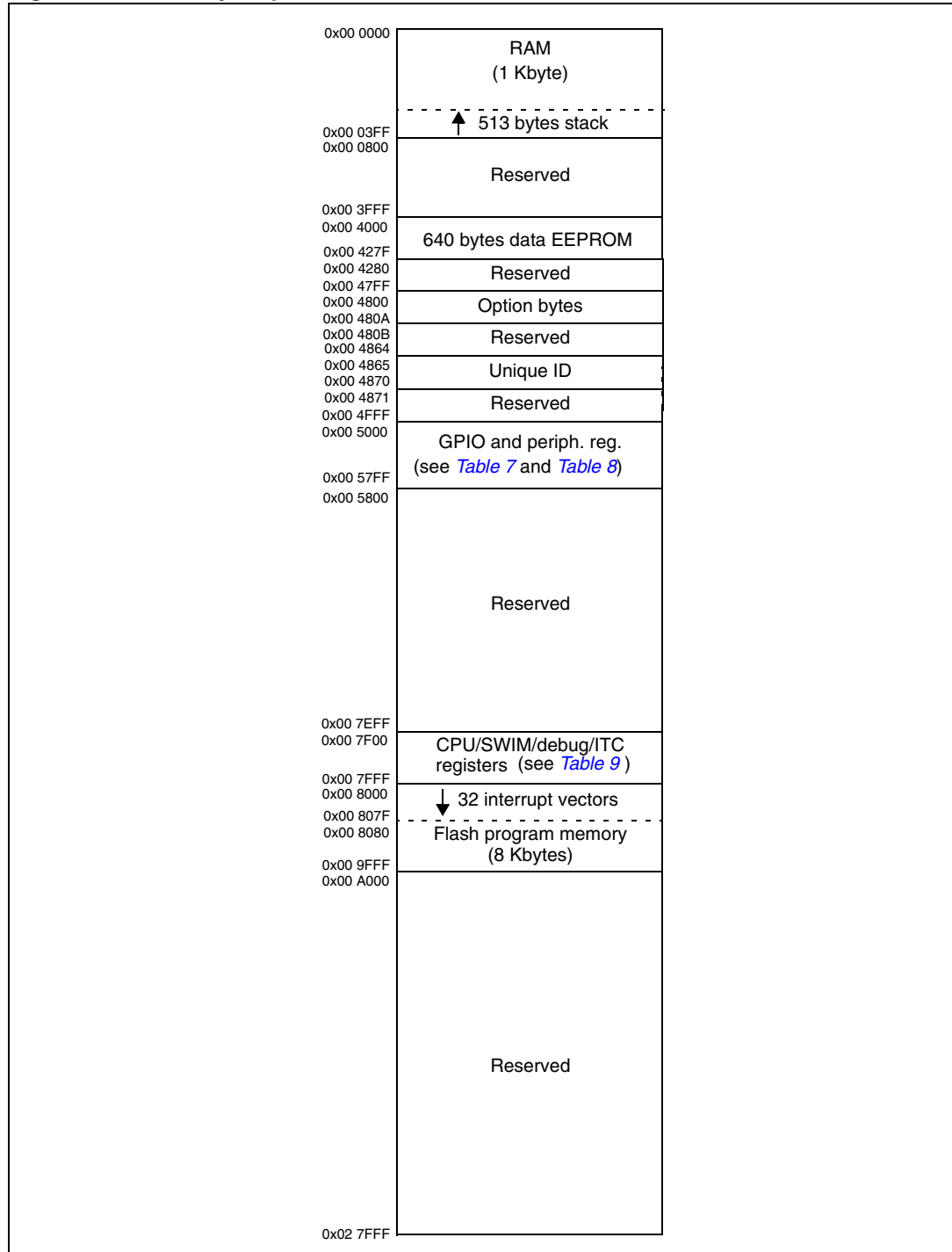
Figure 6. Memory map
