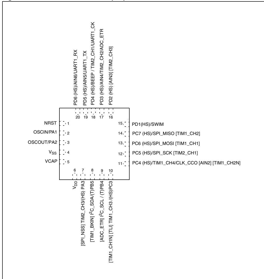
Figure 5. STM8S103F UFQFPN20-pin pinout
