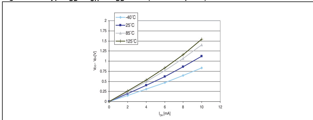
Figure 31. Typ. V_{DD} - V_{OH} @ V_{DD} = 5\text{ V} (standard ports)
