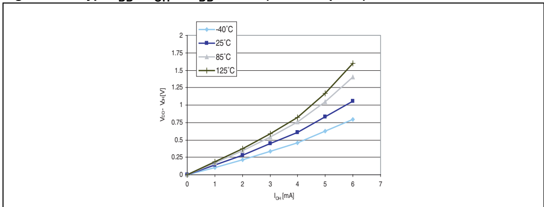
Figure 33. Typ. V_{DD} - V_{OH} @ V_{DD} = 5\text{ V} (high sink ports)
