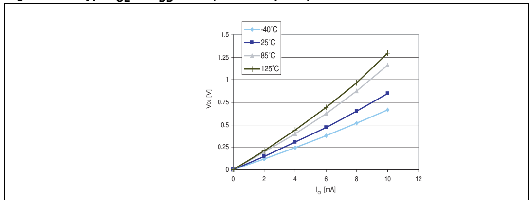
Figure 25. Typ. V OL @ V DD = 5 V (standard ports)
