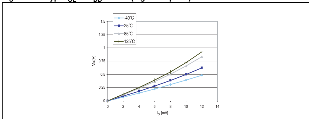
Figure 30. Typ. V_{OL} @ V_{DD} = 3.3\text{ V} (high sink ports)
