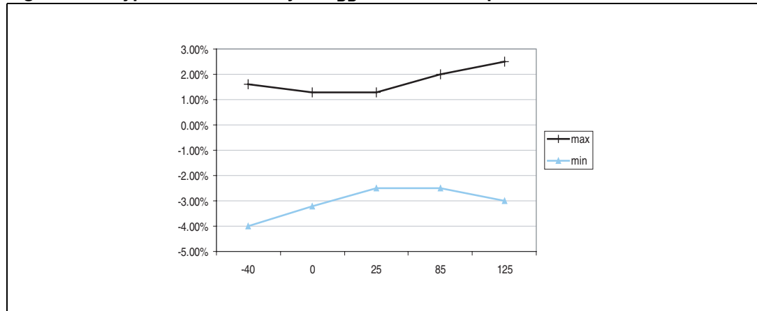
Figure 19. Typical HSI accuracy at V_{DD} = 5\text{ V} vs 5 temperatures
