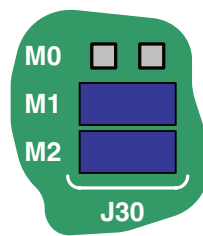
Figure 12-4: Set Mode Pins for SPI Mode
