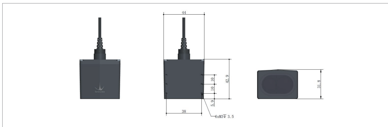
TF03-100 dimensions (Left 1: top view; Left 2: upward view; Left 3: front view) Unit: mm
