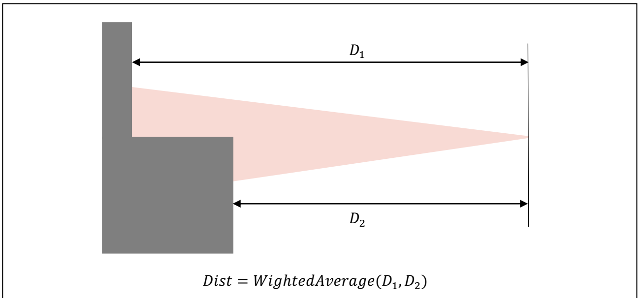
Figure 21 Staircase object
