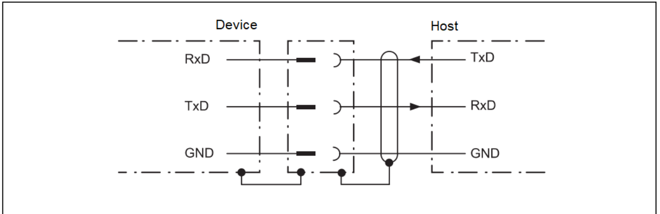
Figure 6 Wiring of the RS-232 interface
