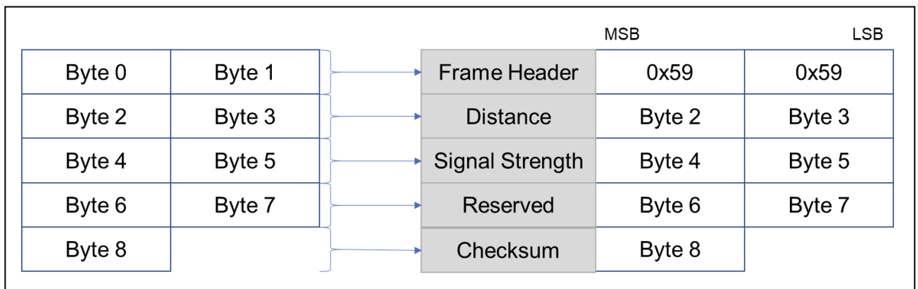
Figure 8 Data communication: User protocol frame format of UART
