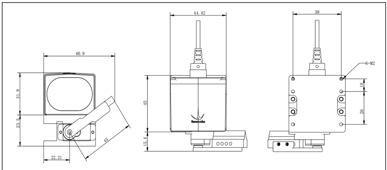
Figure 10 Dimension drawing of self-cleaning module
