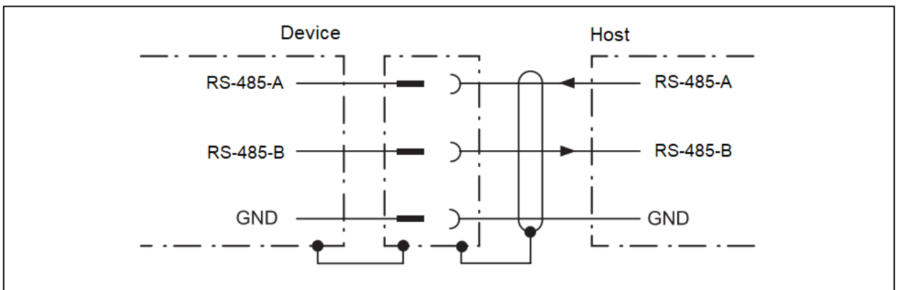
Figure 7 Wiring of the RS-485 interface
