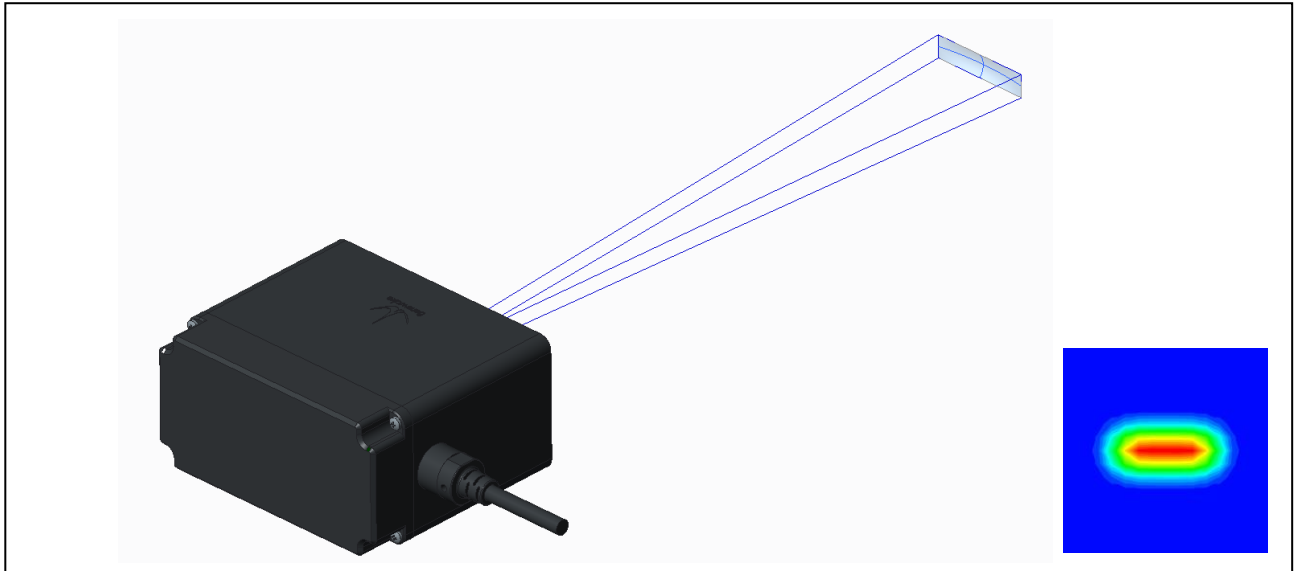
Figure 1 FoV of TF03. Horizontal divergence 0.5^\circ , vertical divergence 0.15^\circ .
