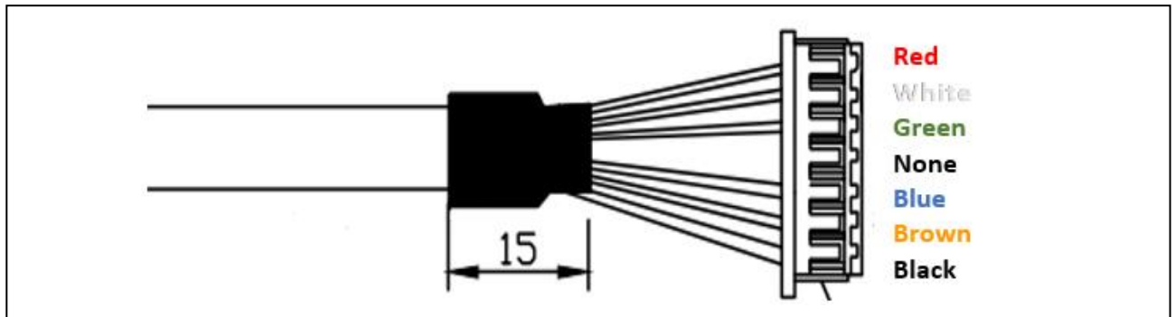
Figure 5 Male connector, Molex SD-51021-007 1.25 W/B-7Pin
