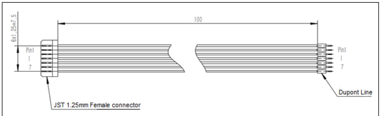
Figure 13 Extension cord for test
