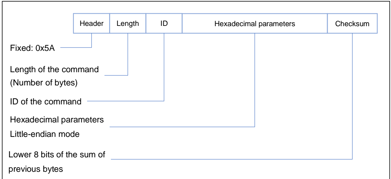
Figure 9 Command syntax of TF03
