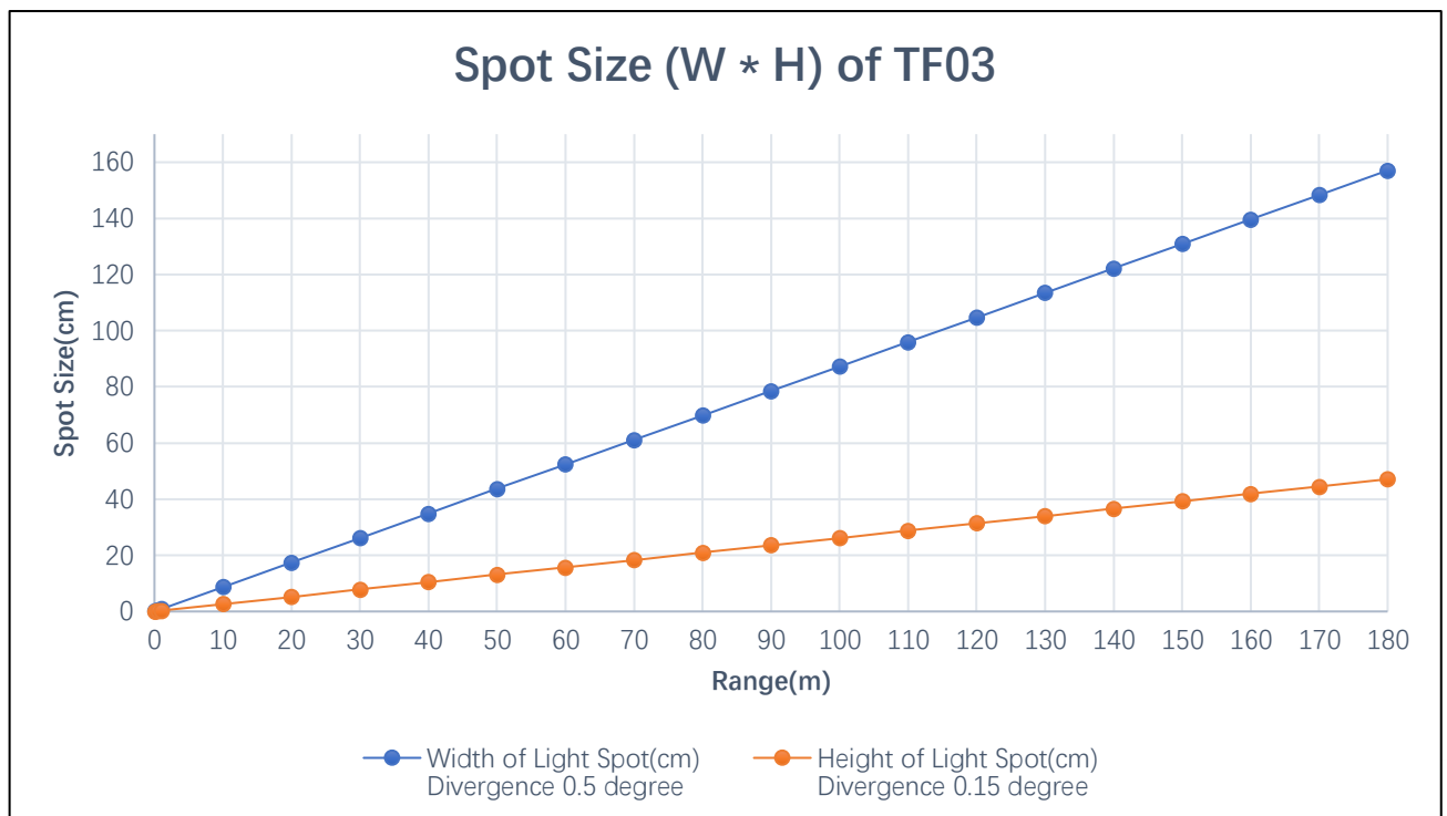
Figure 4 Spot size of TF03 at different range
