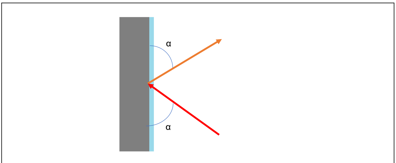
Figure 19 Mirror surfaces
