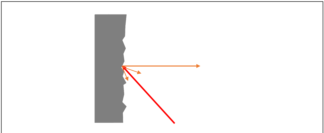
Figure 17 Reflection angle
