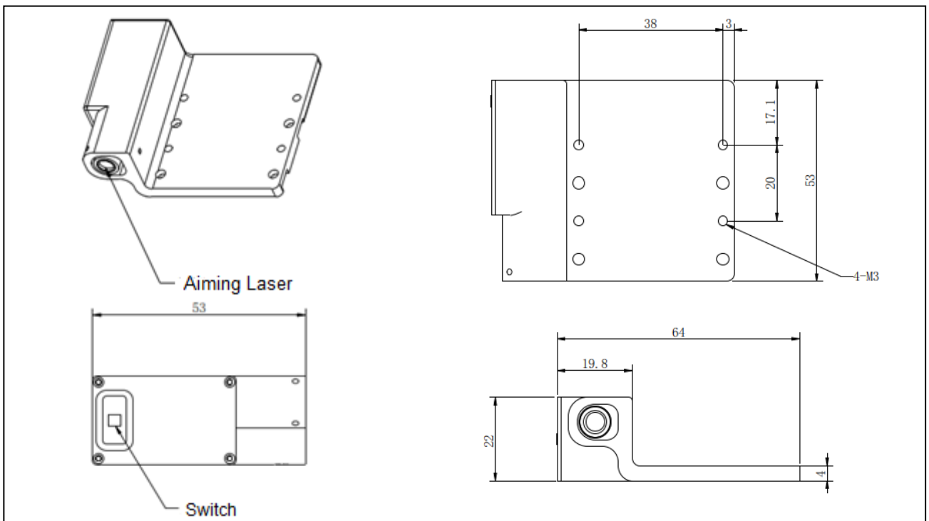
Figure 12 Sketch map of Aiming beam module
