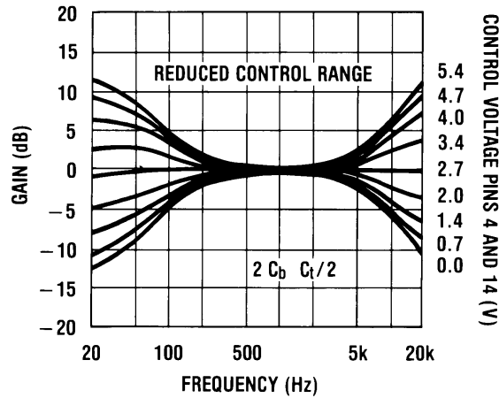
Figure 17. Tone Characteristic (Gain vs Frequency)
