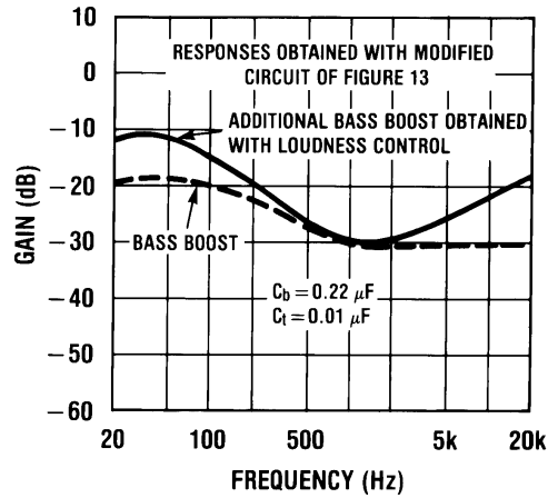
Figure 27. Loudness Compensated Volume Characteristic
