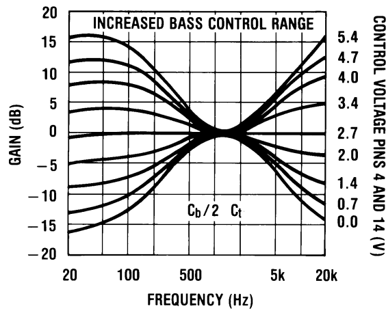
Figure 18. Tone Characteristic (Gain vs Frequency)
