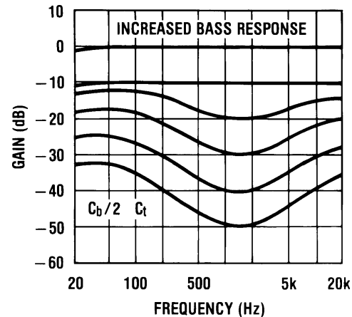
Figure 21. Loudness Compensated Volume Characteristic
