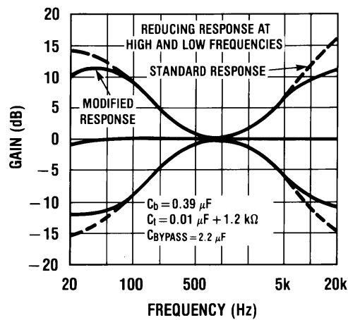
Figure 19. Tone Characteristic (Gain vs Frequency)
