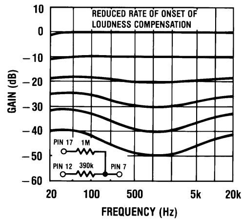
Figure 24. Loudness Compensated Volume Characteristic
