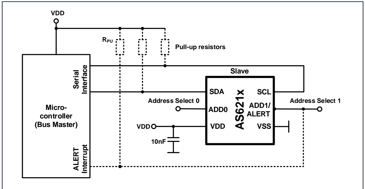
Figure 34: Application Example
