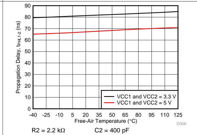
Figure 11. t_{PHL1-2} Propagation Delay vs Free-Air Temperature
