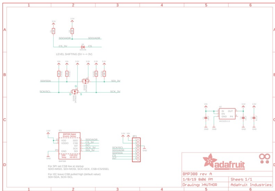
Schematic and Fab Print for BMP388 Original Version
