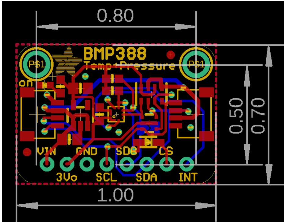
Schematic and Fab Print for BMP388 Original Version
