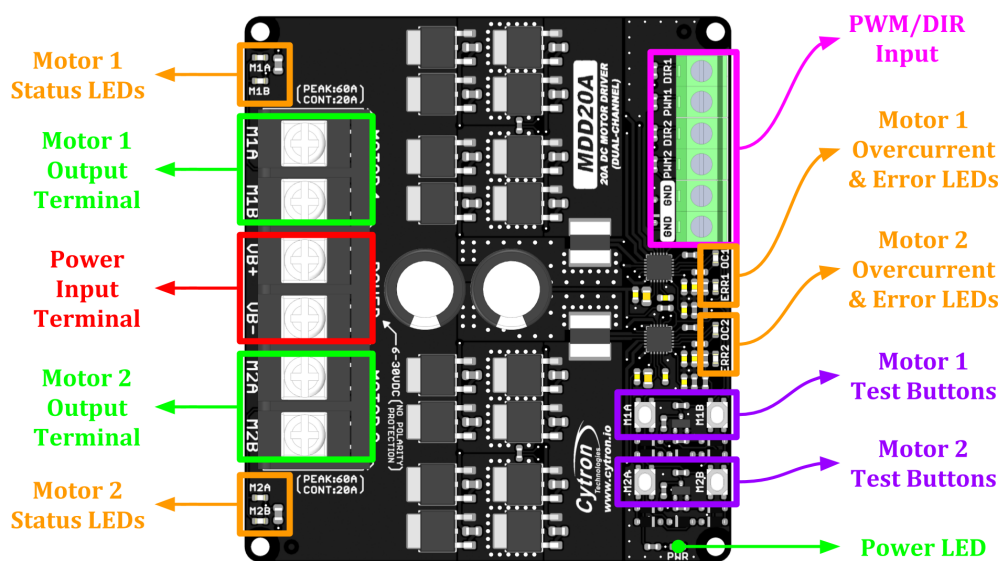
Figure 1: MDD20A Board Functions
