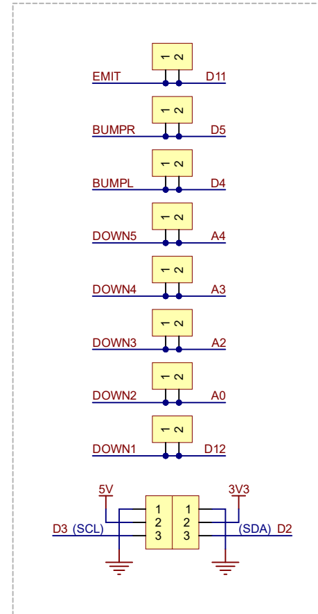
Front expansion header
