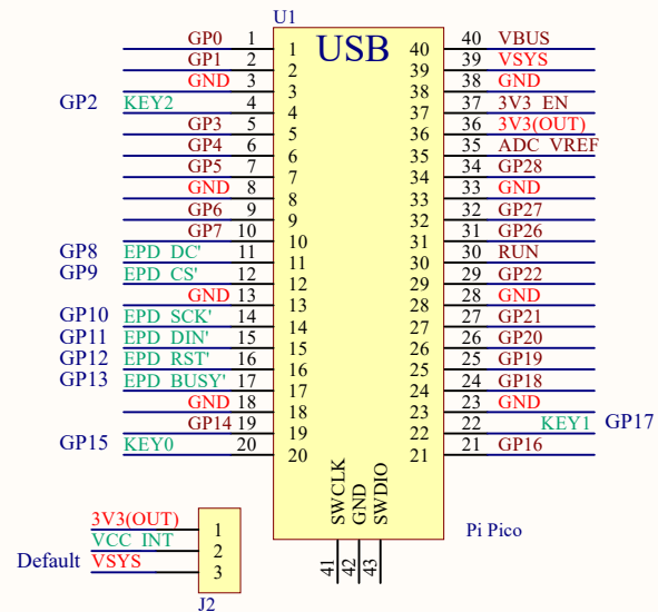
Connector_Pico
