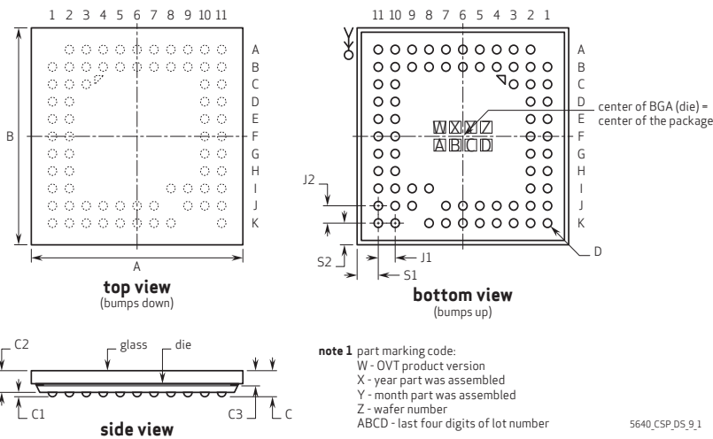
figure 9-1 package specifications
