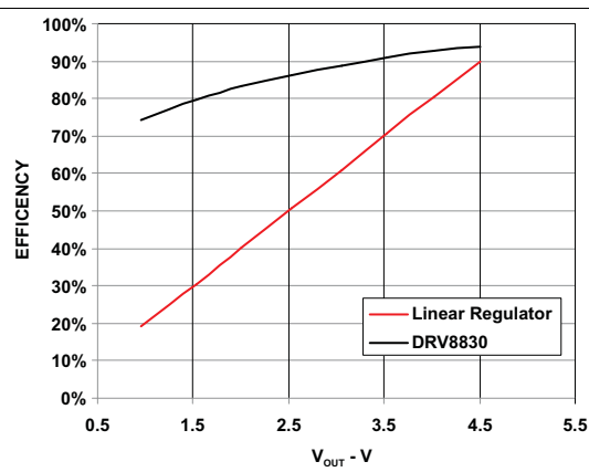
Figure 4. Efficiency vs Output Voltage ( V_{IN} = 5\text{ V} , I_{OUT} = 500\text{ mA} )
