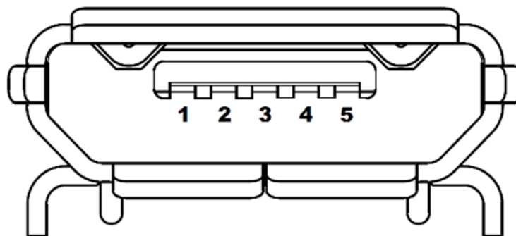
Figure 6. CN11 ST-LINK USB Micro-B connector pinout
