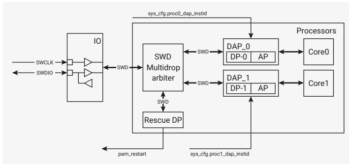
Figure 10. RP2040 Debugging
