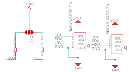
Qwiic Connector
