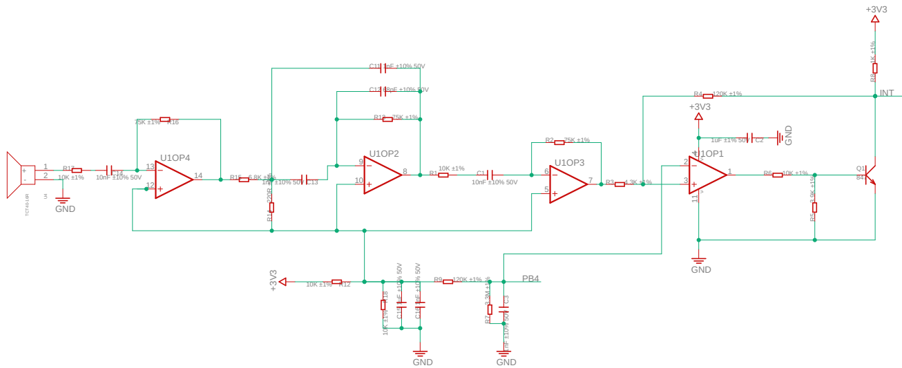
Ultrasound reception
