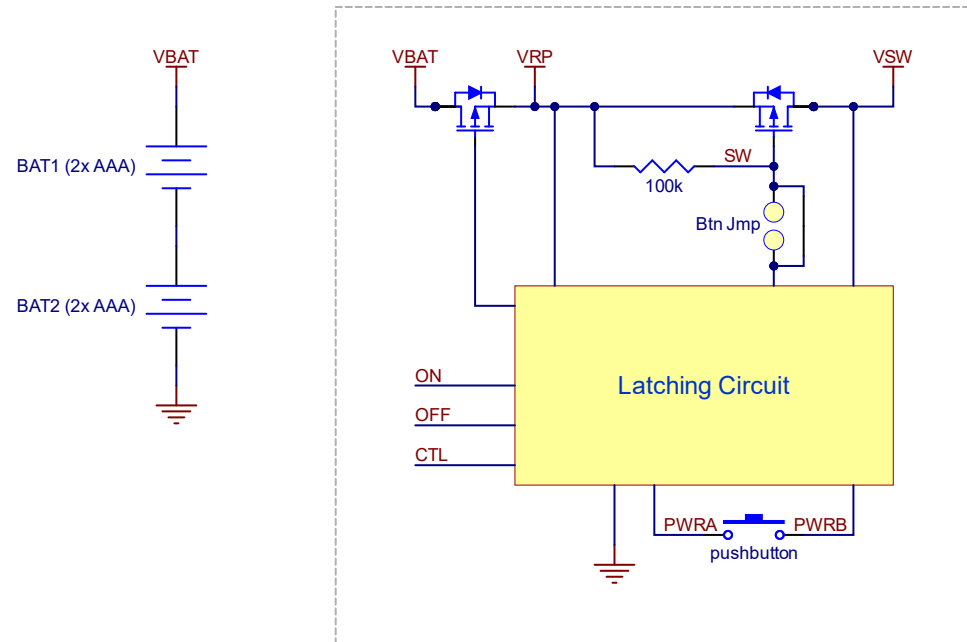
Simplified switch schematic
