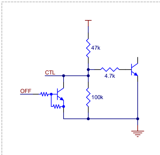
Input structure of OFF and CTL inputs
