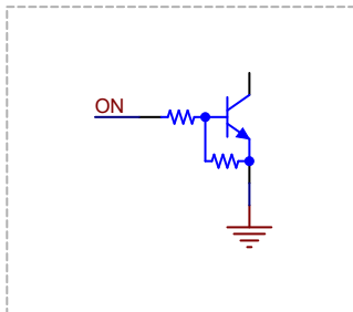
Input structure of ON input
