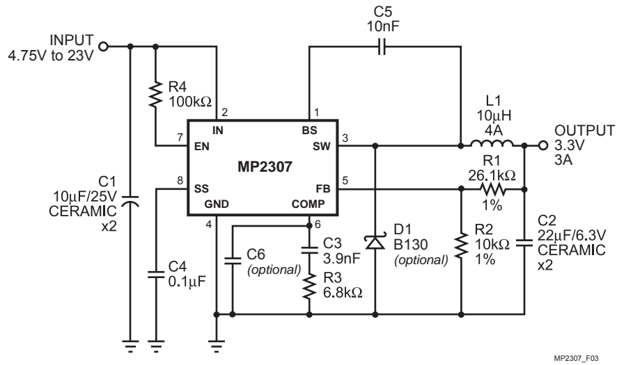
Figure 3—MP2307 with 3.3V Output, 22µF/6.3V Ceramic Output Capacitor
