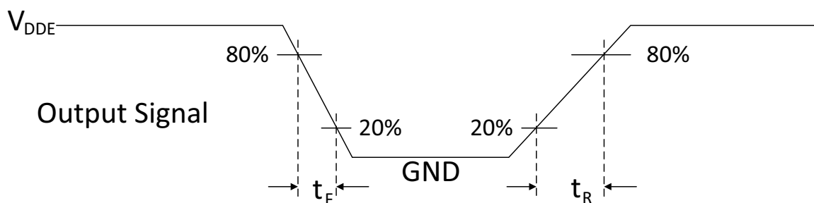
Fig 10. Output timing measurement condition
