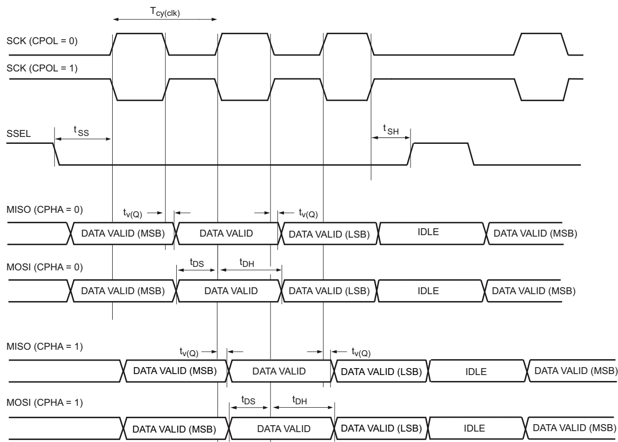
Fig 12. SPI slave interface timings
