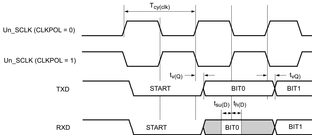
Fig 13. USART interface timings
