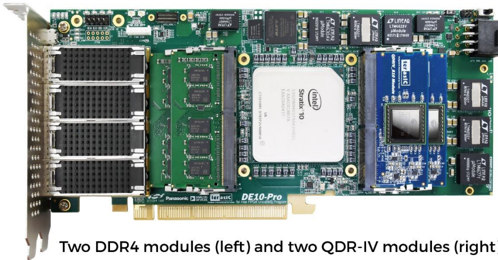
Figure 2-13 Connection between the DDR4 and Stratix 10 GX/SX FPGA
