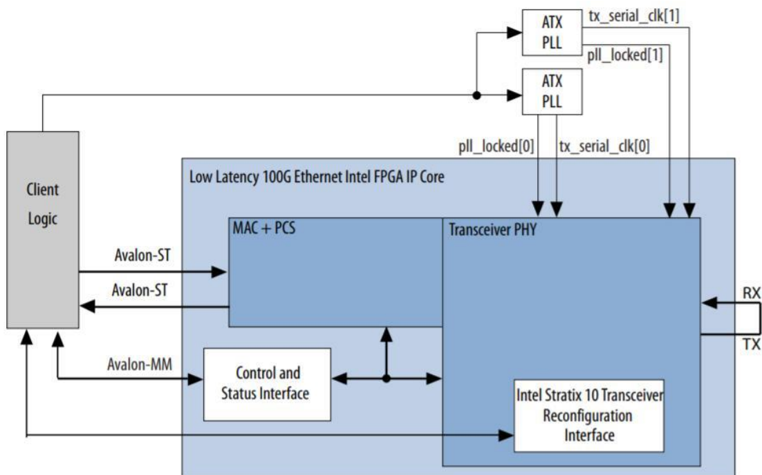
Figure 9-6 Block diagram of 100GbE demo
