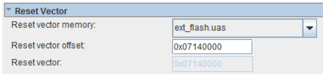
Figure 4-7 Factory Software Reset Vector Settings for NIOS II Processor
