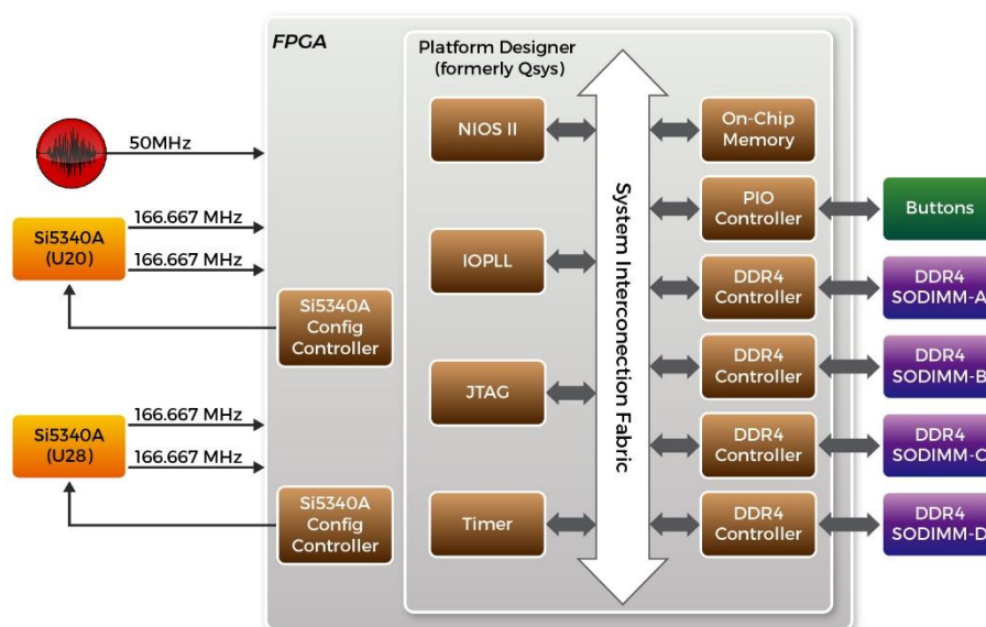
Figure 6-2 Block diagram of the DDR4 Basic Demonstration
