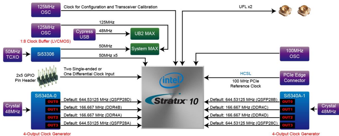
Figure 5-1 The clock tree of the DE10-Pro
