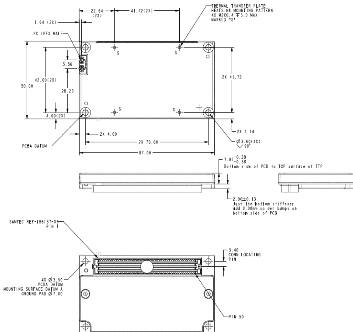
Figure 7 TX2 SOM Package Outline with Dimensions
