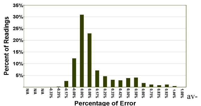
MB7554 without External Temperature Sensor
