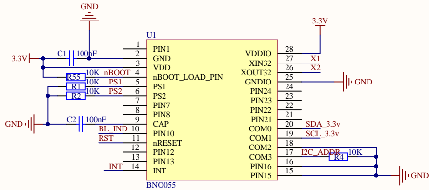
I2C address 0x28 BNO055
