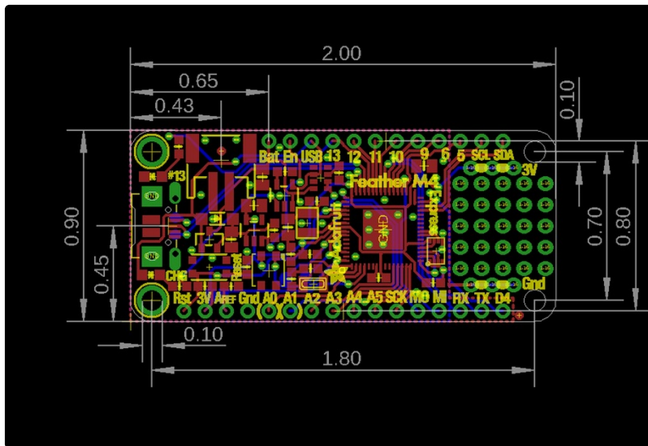
Pinout Diagram
