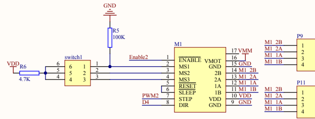
DRIVER_PART
