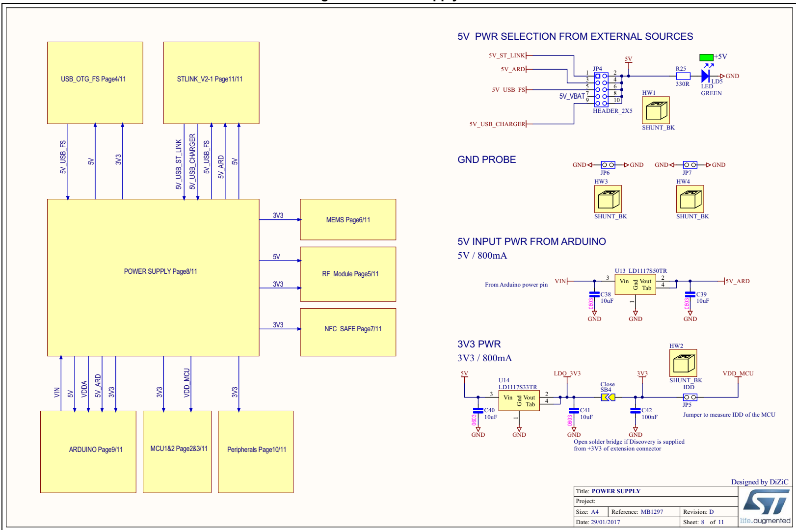
Figure 29. Power supply
