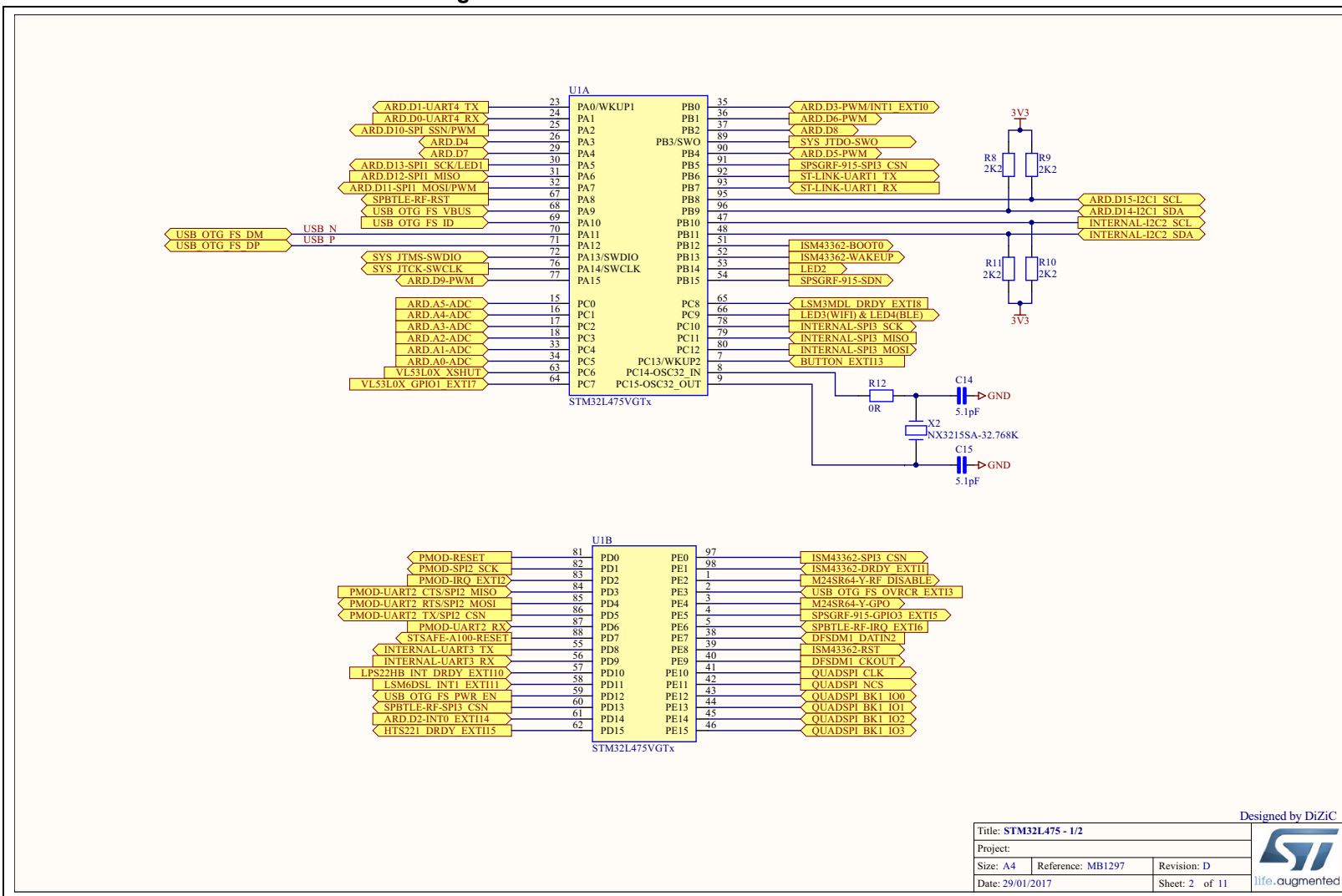
Figure 23. STM32L475VG microcontroller
