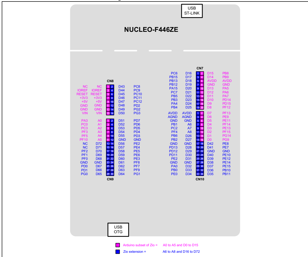
Figure 14. NUCLEO-F446ZE
