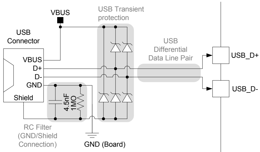
Figure 38-15. Protected USB Interface Example Schematic
