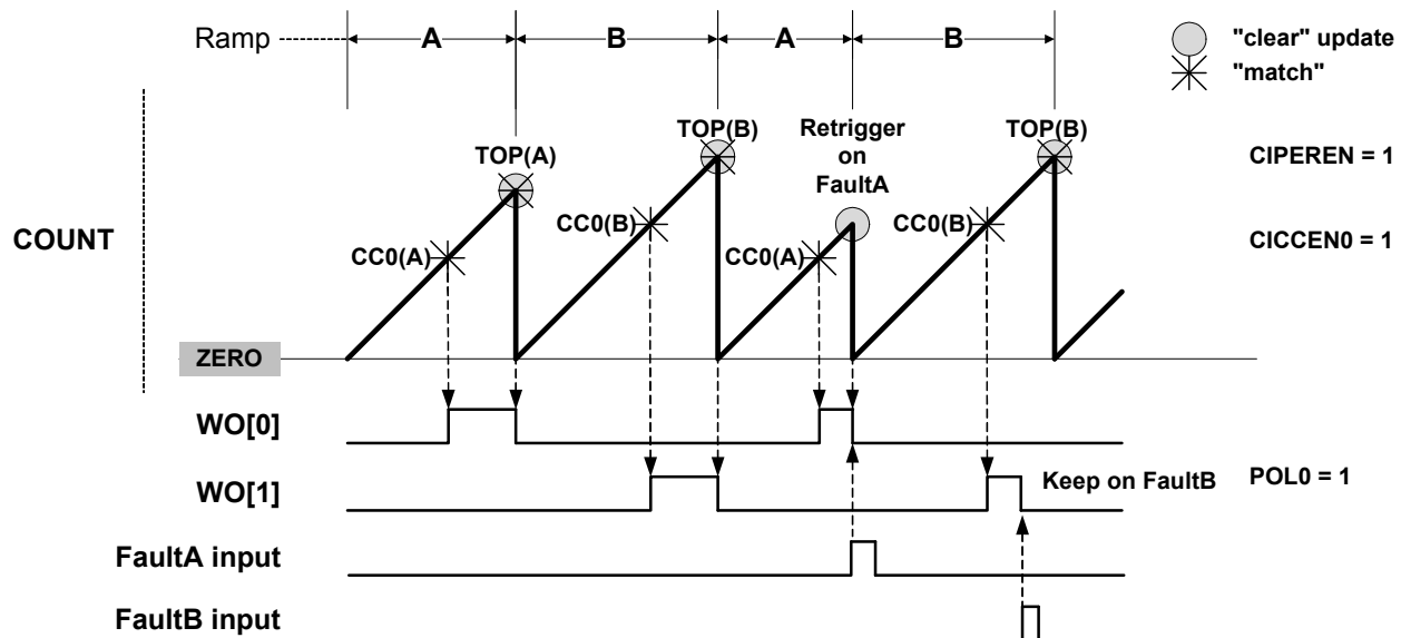
Figure 30-21.RAMP2 Alternate Operation
