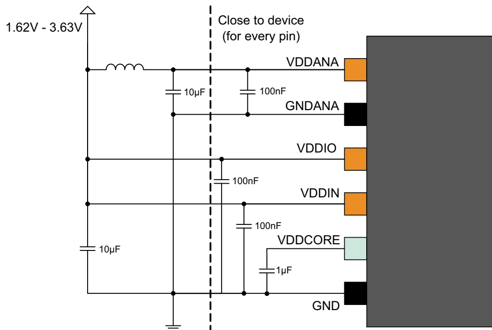
Figure 38-1. Power Supply Schematic
