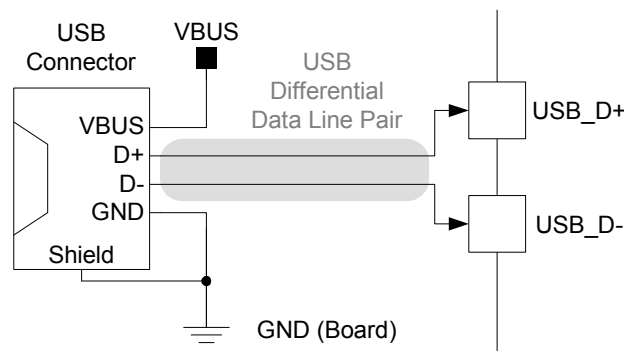
Figure 38-14. Low Cost USB Interface Example Schematic
