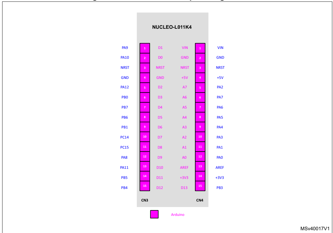
Figure 7. NUCLEO-L011K4 pin assignment
