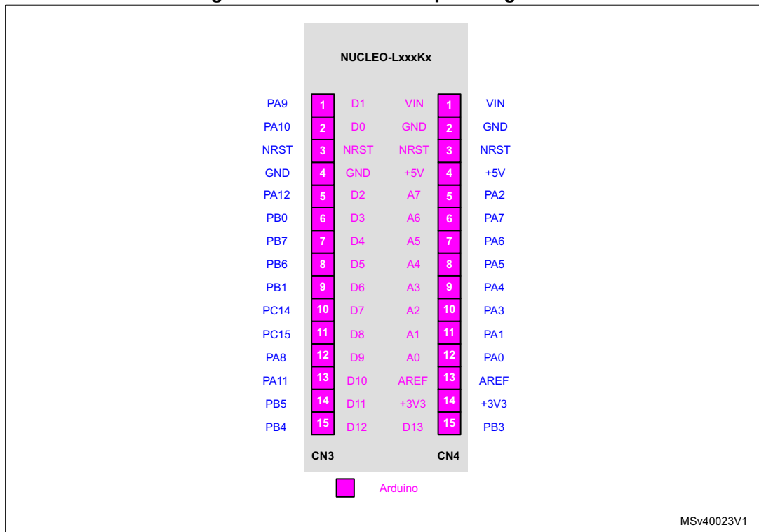
Figure 8. NUCLEO-L031K6 pin assignment
