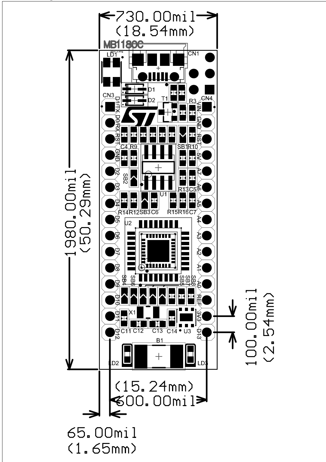
Figure 12. Nucleo-32 board mechanical dimensions in millimeter
