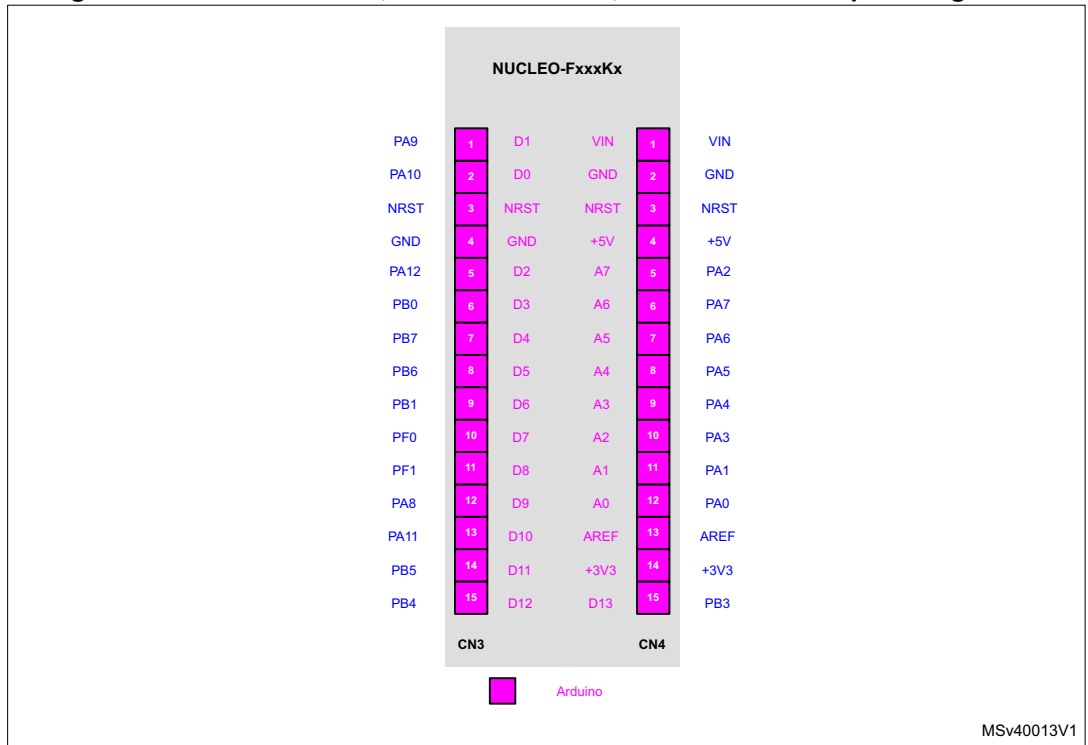
Figure 6. NUCLEO-F031K6, NUCLEO-F042K6, NUCLEO-F303K8 pin assignment
