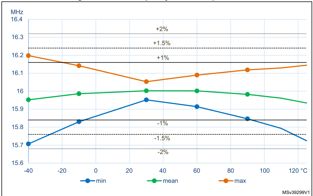
Figure 18. HSI16 frequency versus temperature
