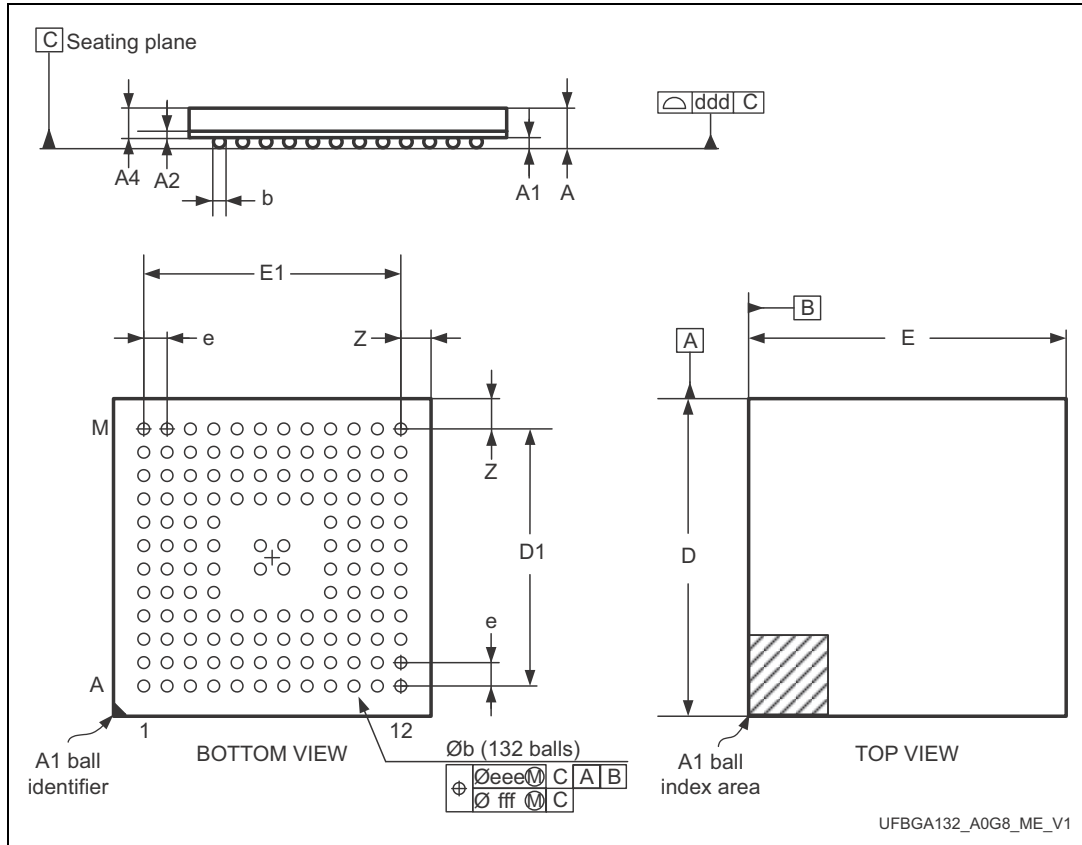
Figure 50. UFBGA132 - 132-ball, 7 x 7 mm ultra thin fine pitch ball grid array package outline
