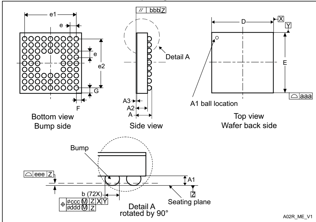
Figure 56. WLCSP72 - 72-ball, 4.4084 x 3.7594 mm, 0.4 mm pitch wafer level chip scale package outline
