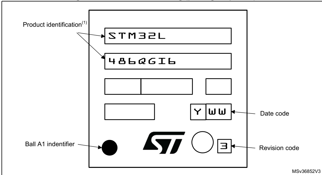
Figure 52. UFBGA132 marking (package top view)
