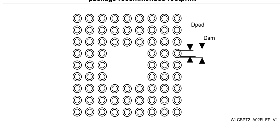
Figure 57. WLCSP72 - 72-ball, 4.4084 x 3.7594 mm, 0.4 mm pitch wafer level chip scale package recommended footprint
