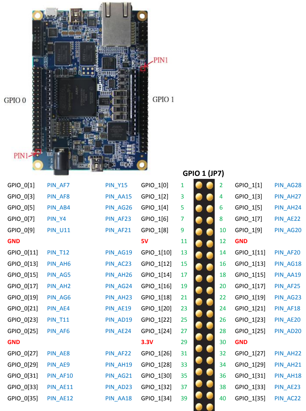
Figure 3-18 GPIO Pin Arrangement
