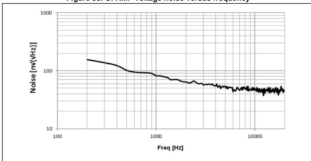
Figure 53. OPAMP voltage noise versus frequency
