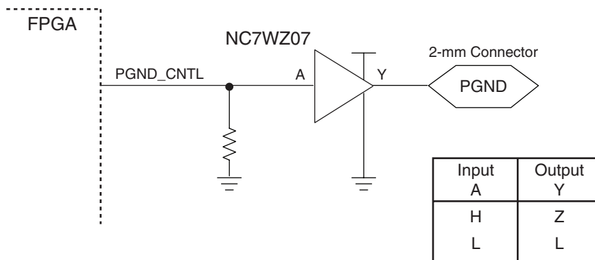
Figure 23: PGND Signal
