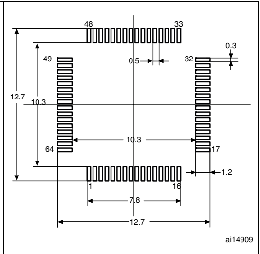
Figure 40. Recommended footprint (1)(2)
