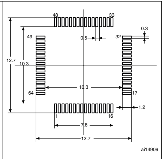
Figure 36. Recommended footprint (1)(2)
