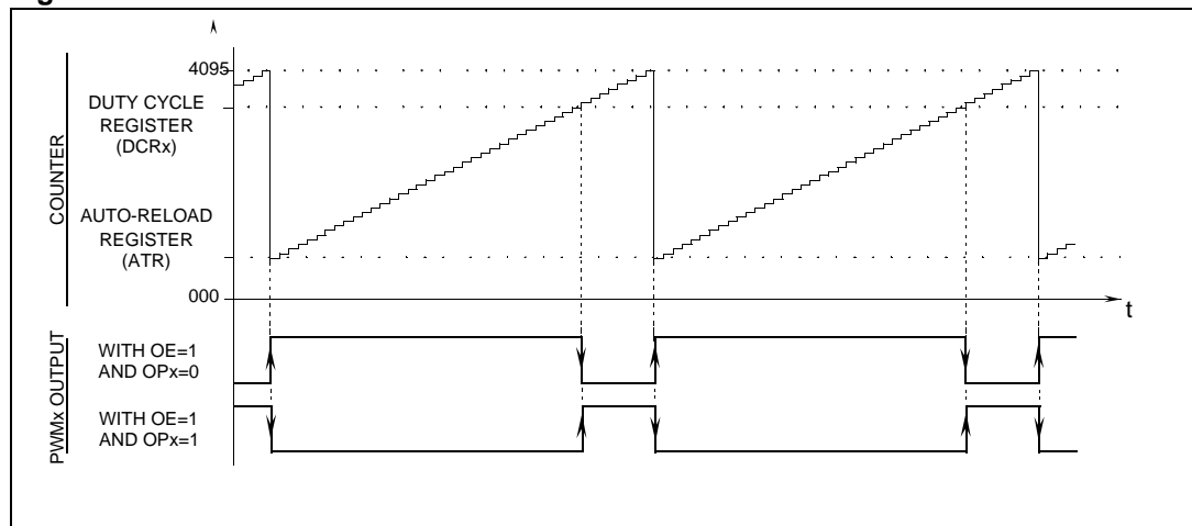
Figure 38. PWM function
