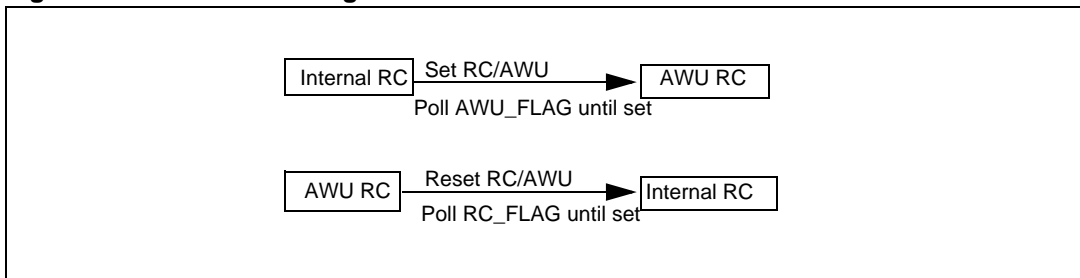
Figure 11. Clock switching
