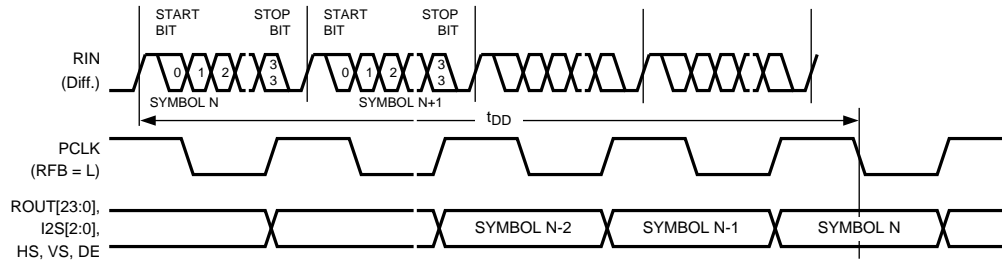
Figure 4. Delay - Latency
