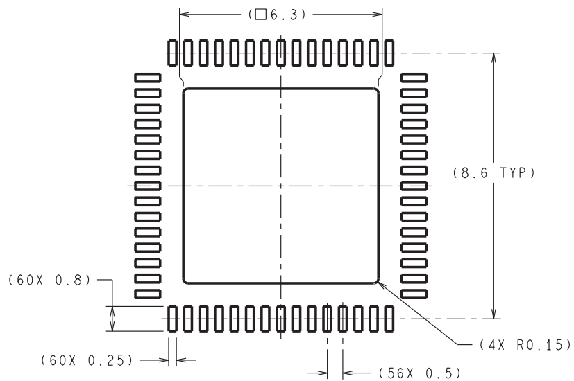
Figure 29. 60-Pin WQFN Stencil Example of Via and Opening Placement
