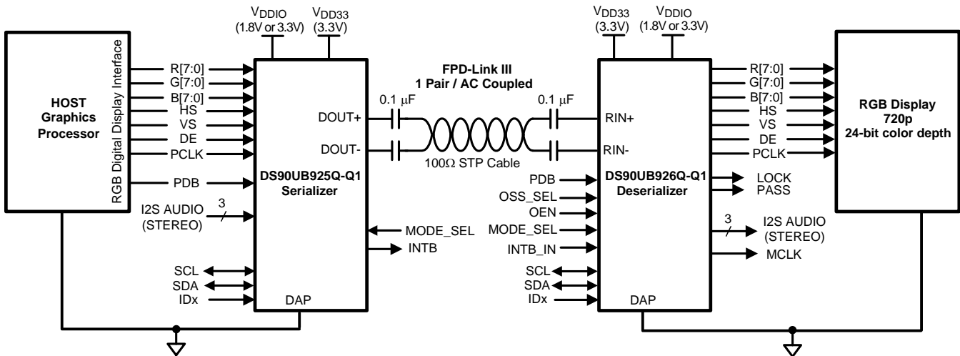
Figure 25. Typical Display System Diagram
