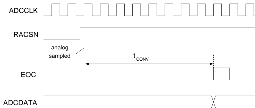
Figure 8 Timing diagram single step conversion.
