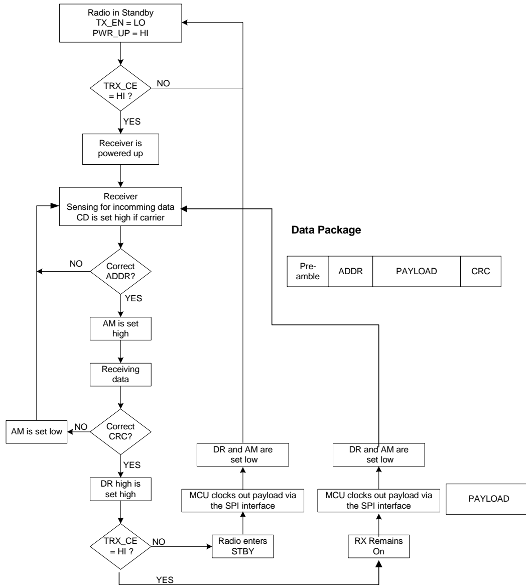
Figure 6 Flowchart ShockBurst™ receive of nRF905.
