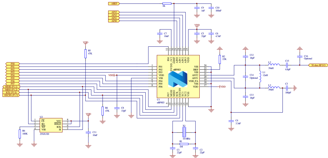
Figure 38 433MHz operating nRF9E5 application schematic, single ended connection to 50Ω antenna by using a differential to single ended matching network.
