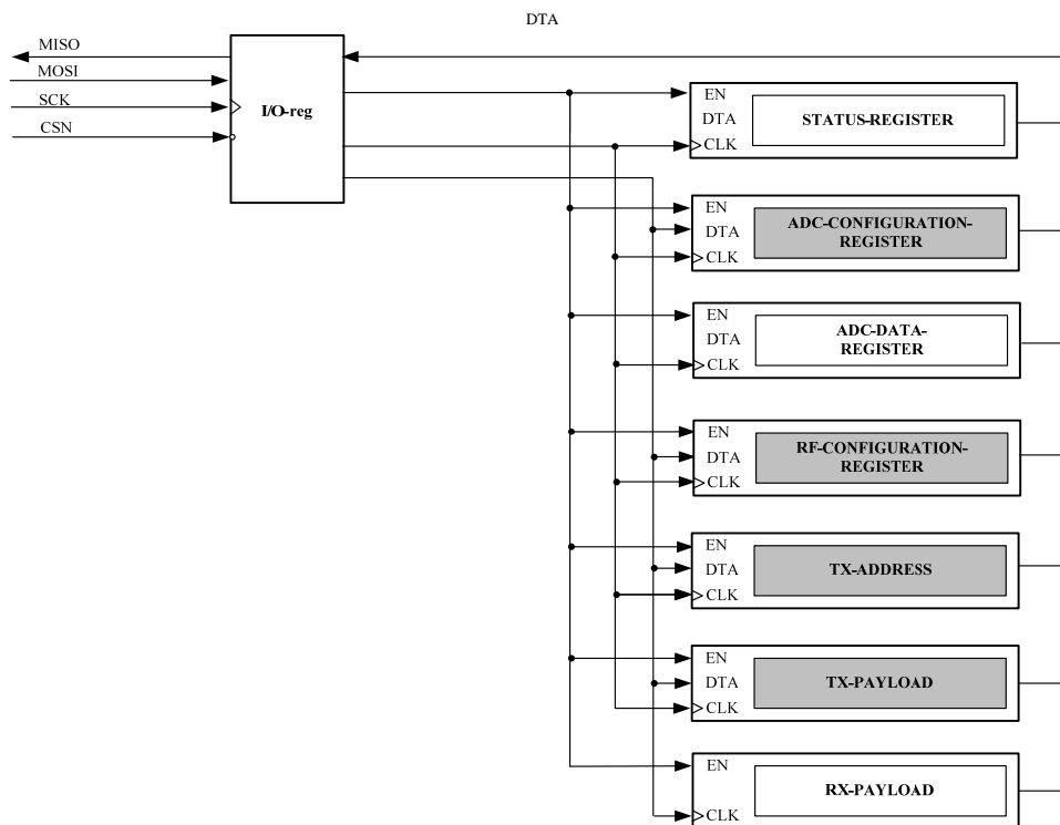
Figure 10 SPI – interface composed of seven internal registers.
