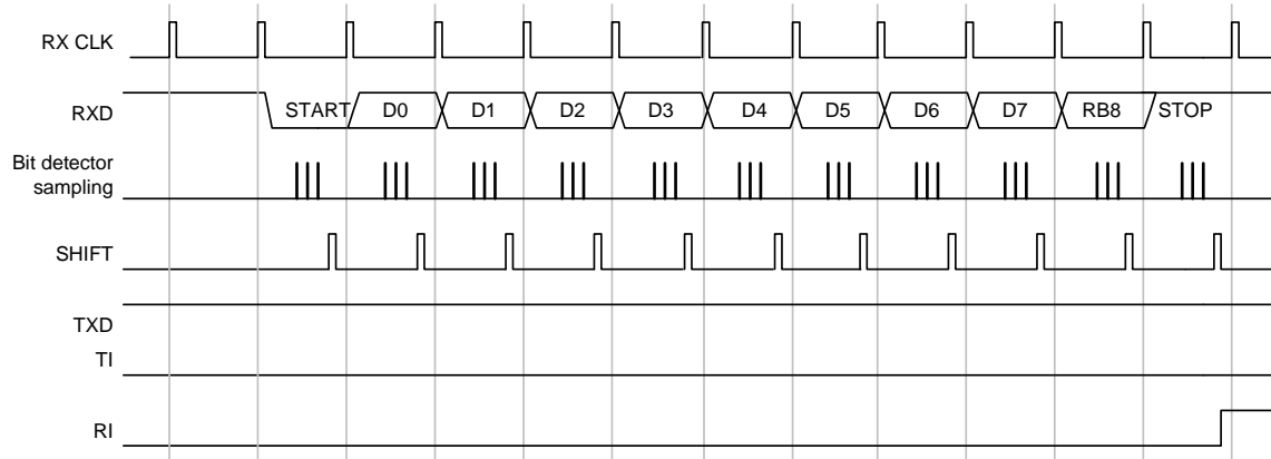
Figure 33 Serial port Mode 3 Receive Timing.
