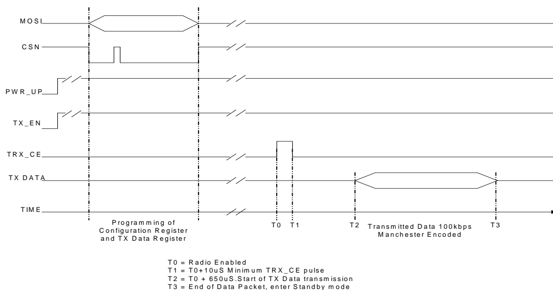
Figure 13 Timing diagram for standby to transmit.
