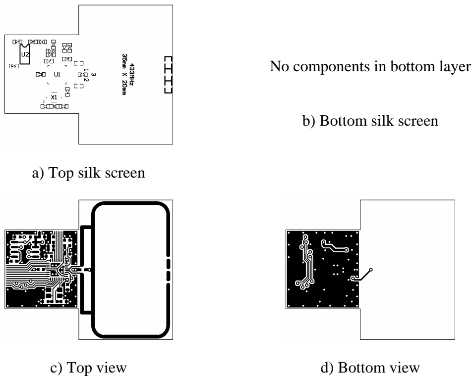
Figure 37 PCB layout example for nRF9E5, differential connection to a loop antenna.
