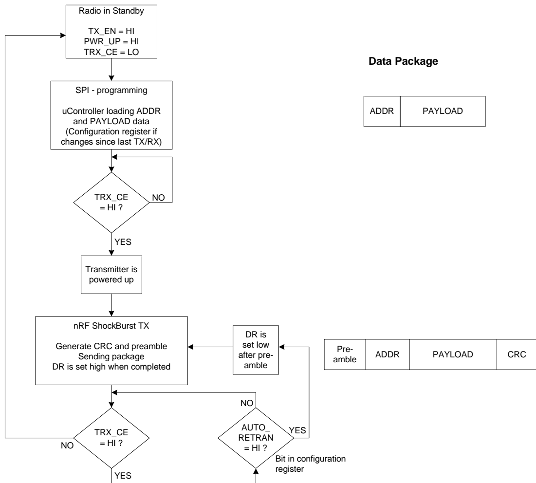
Figure 5 Flowchart ShockBurst™ transmit of nRF905.
