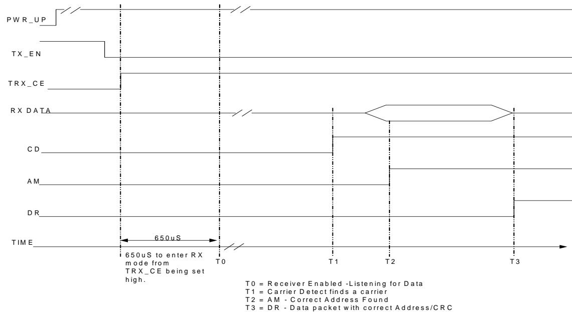
Figure 14 Timing diagram for standby to receiving.
