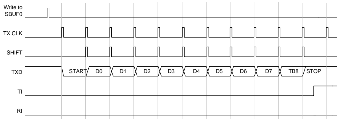
Figure 32 Serial port Mode 3 Transmit Timing.
