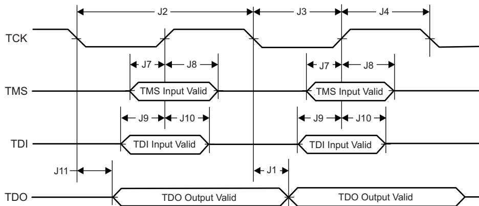
Figure 4-18. JTAG Timing
