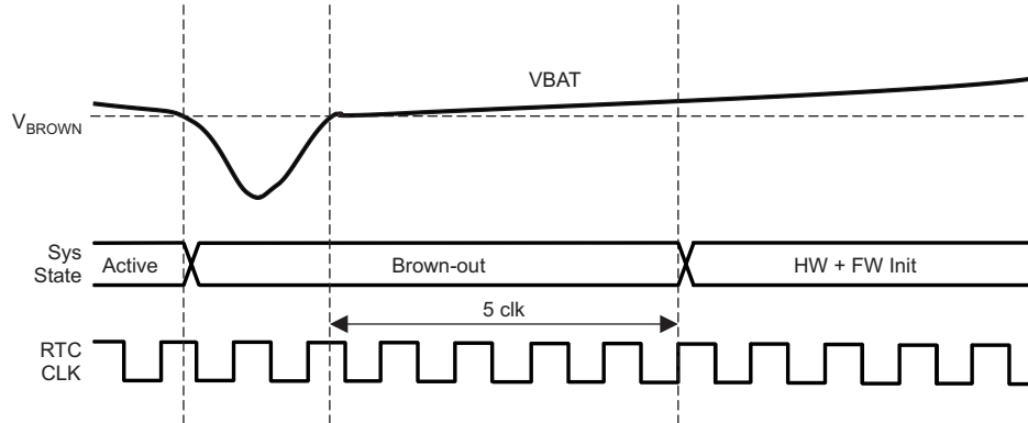
Figure 4-1. Brown-Out Timing Diagram
