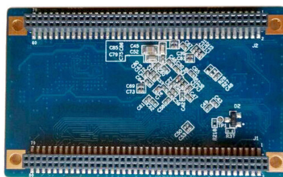
Figure 1-2 MYC-IMX28X Bottom-view
