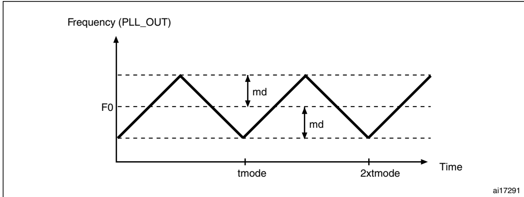
Figure 27. PLL output clock waveforms in center spread mode
