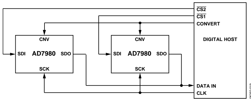
Figure 35. 4-Wire CS Mode Without Busy Indicator Connection Diagram
