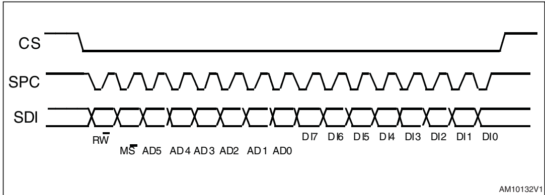
Figure 11. Magnetometer SPI write protocol
