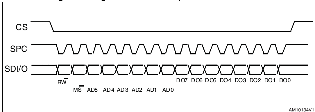
Figure 13. Magnetometer SPI read protocol in 3-wire mode
