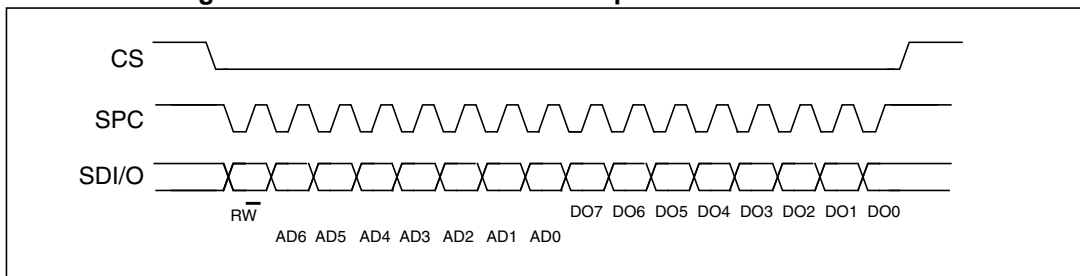
Figure 10. Accelerometer SPI read protocol in 3-wire mode
