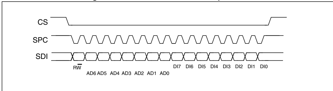
Figure 8. Accelerometer SPI write protocol
