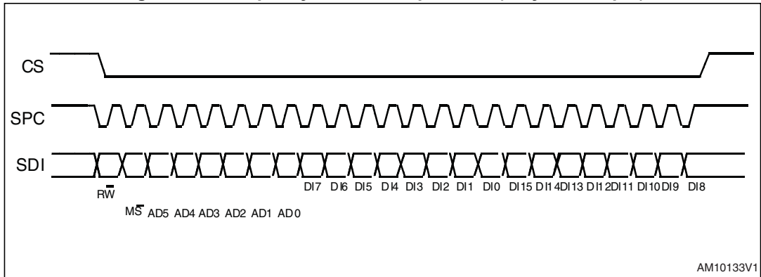
Figure 12. Multiple byte SPI write protocol (2-byte example)
