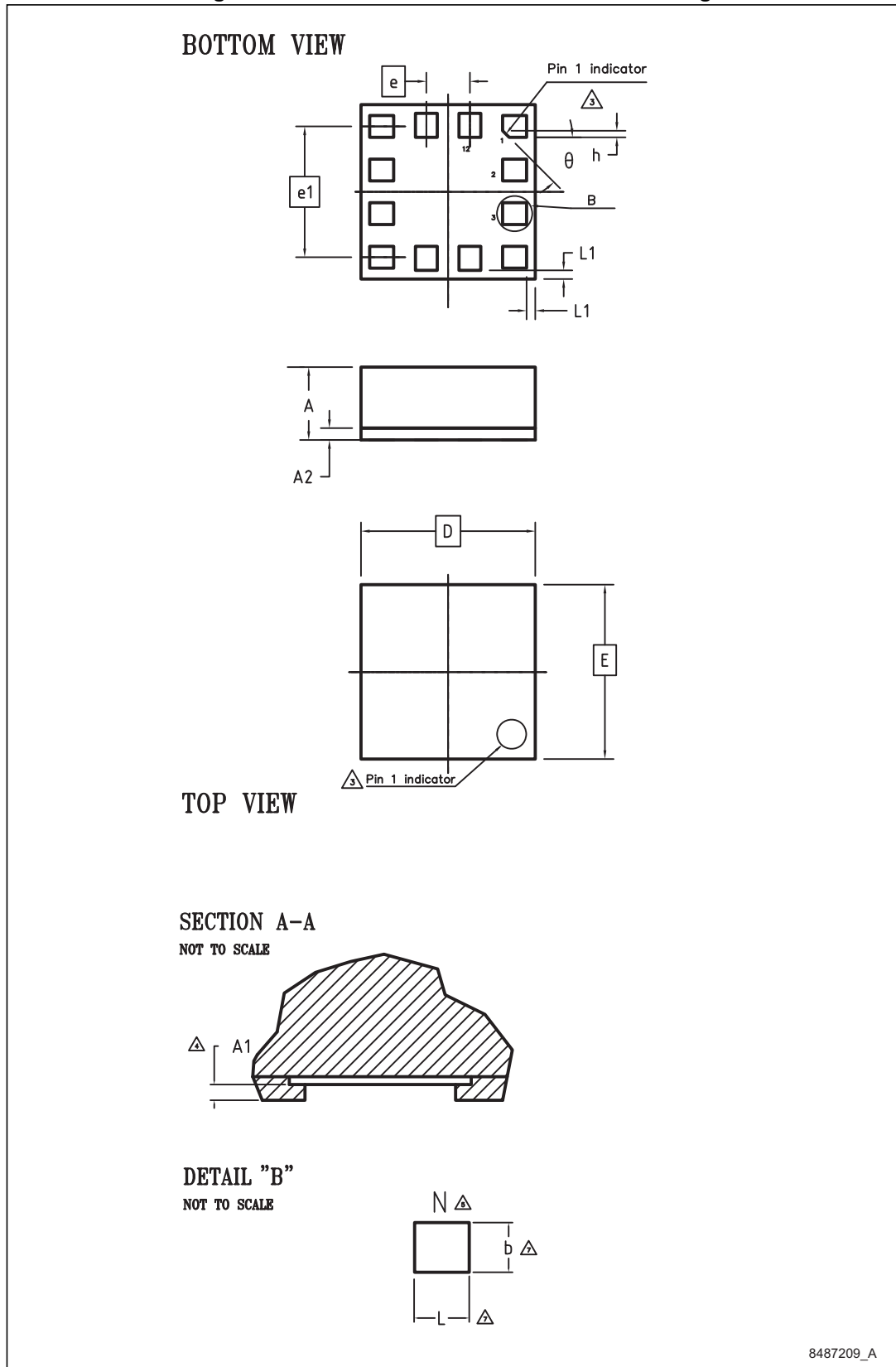
Figure 14. LGA-12 2x2x1 mm mechanical drawing
