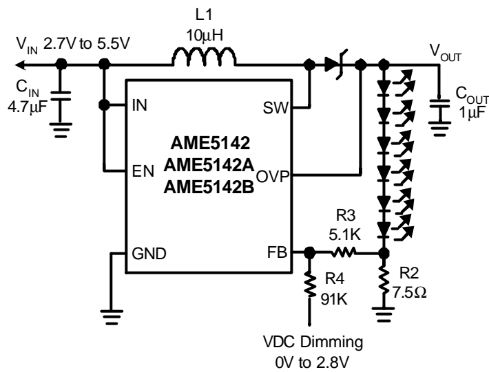
Figure 6. Dimming Control Using a DC Voltage
