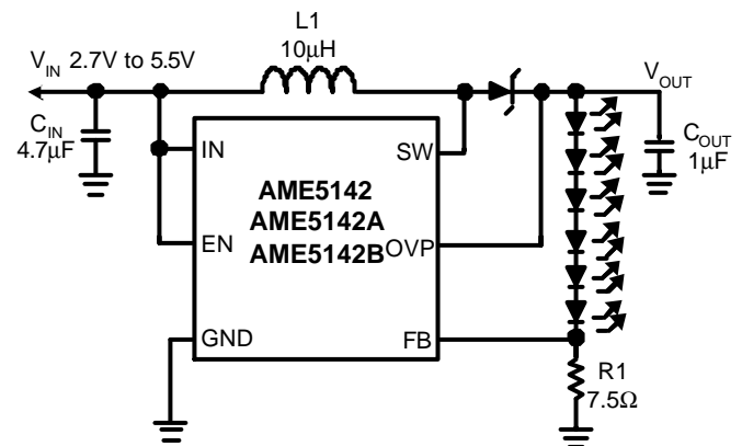
Figure 3: Circuit For Driving 6 White LEDs
