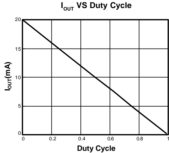
Figure 7. Dimming Control Using a Filtered PWM Signal
