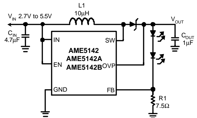
Figure 1: Circuit For Driving 2 White LEDs
