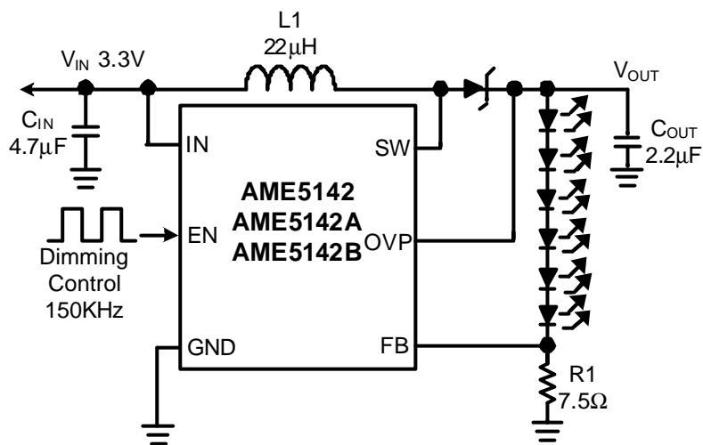
Figure 5. PWM Dimming Control Using the EN Pin
