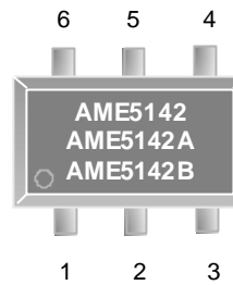
SOT-26/TSOT-26 (Recommend) Top View
