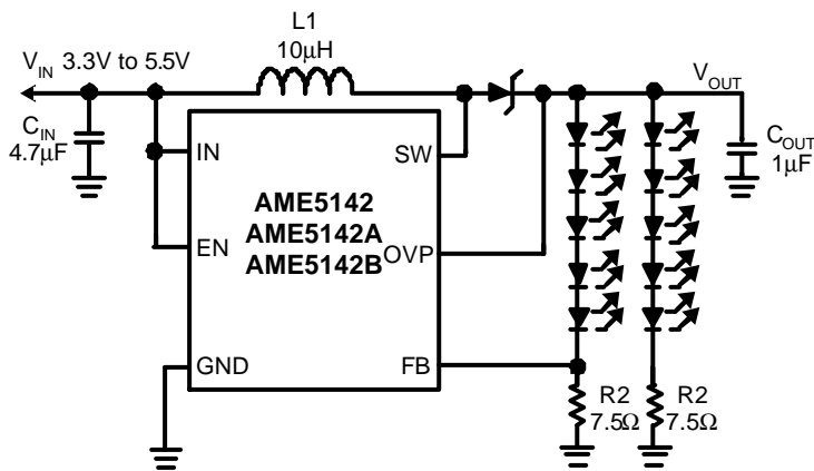
Figure 13: Circuit For Driving 2 Strings of 5 White LEDs
