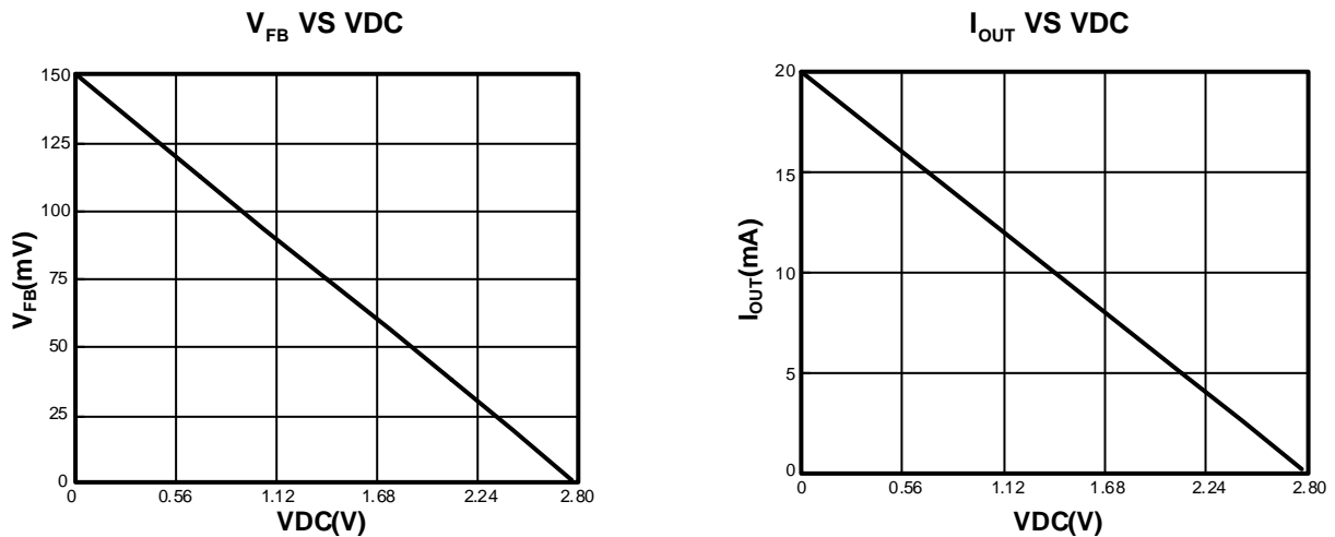
Figure 6. Dimming Control Using a DC Voltage
