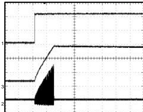
Start up into Openload AME5142B
