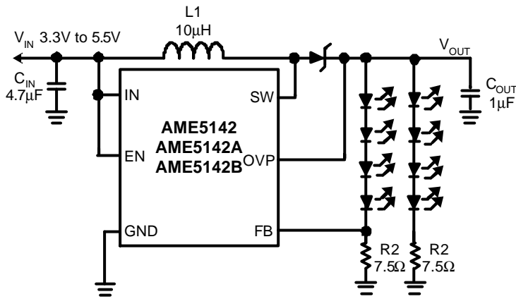
Figure 11: Circuit For Driving 2 Strings of 4 White LEDs
