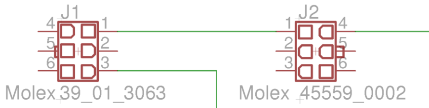
Figure 1. Power Adapter for Digilent SWPS-60W (connector end view).
