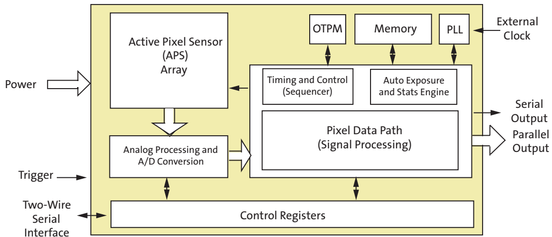
Figure 1: Block Diagram
