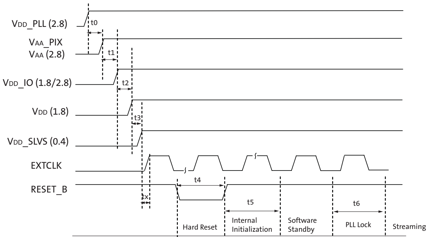
Figure 34: Power Up
