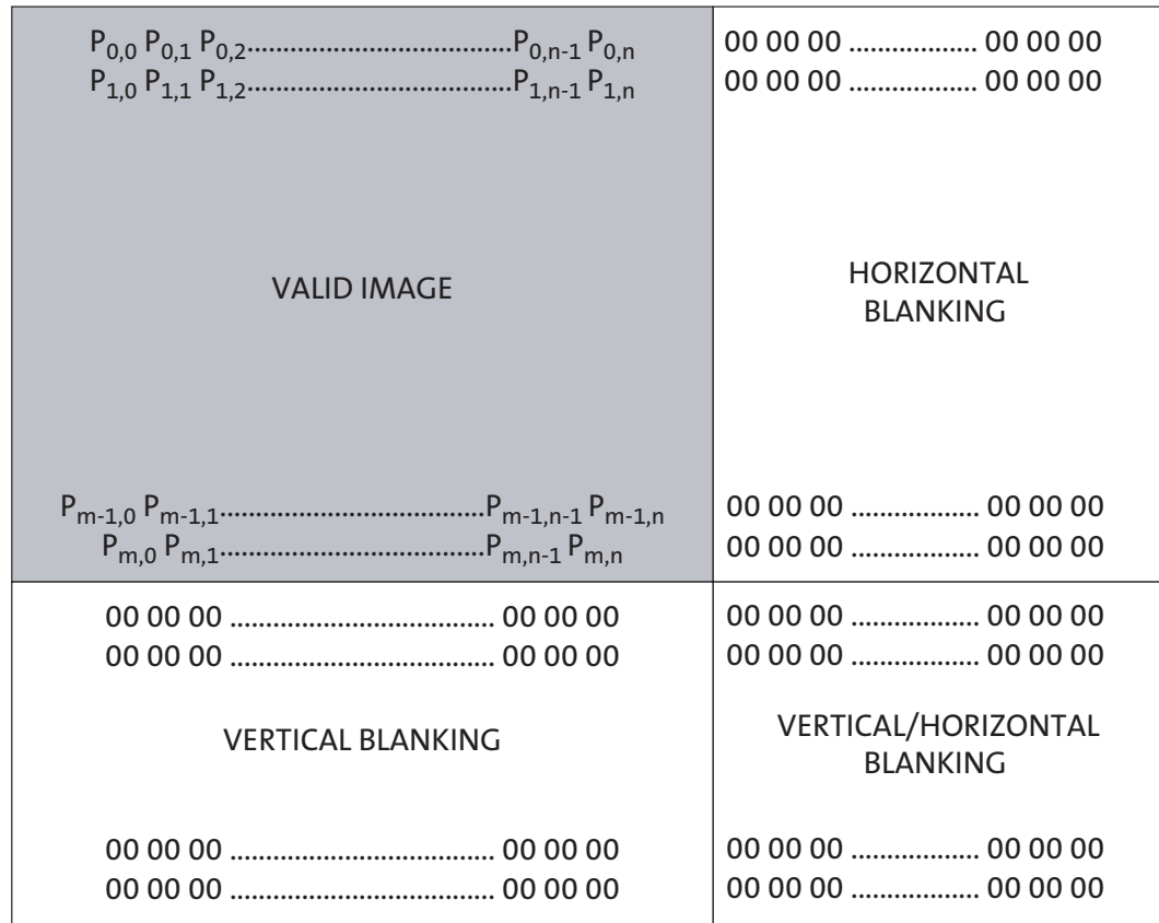
Figure 9: Spatial Illustration of Image Readout
