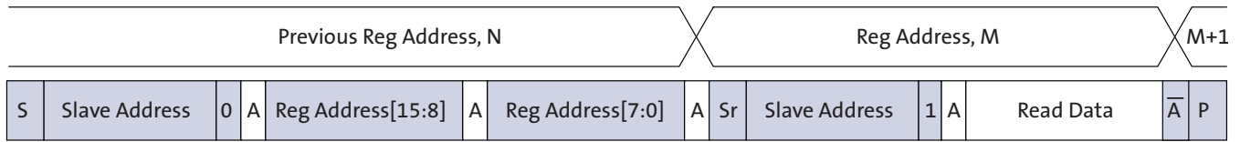
Figure 21: Single READ from Random Location
