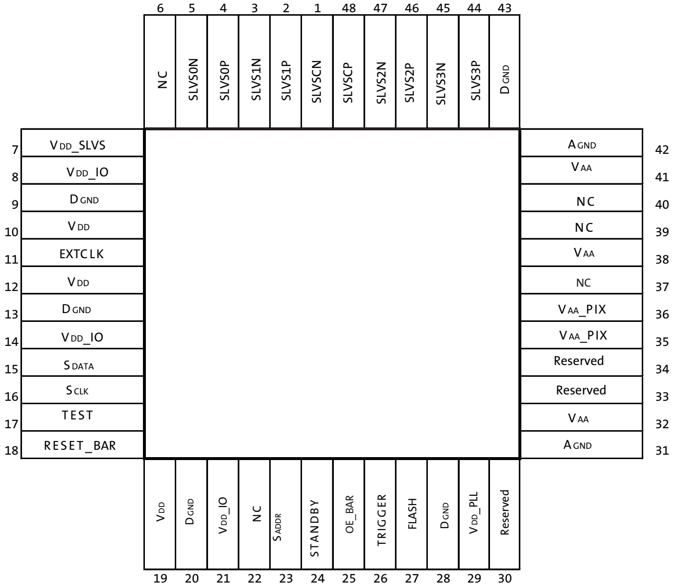
Figure 5: 48 iLCC Package, HiSPi Output
