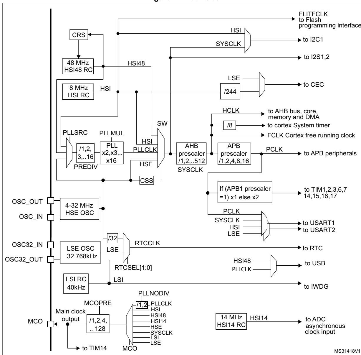
Figure 2. Clock tree
