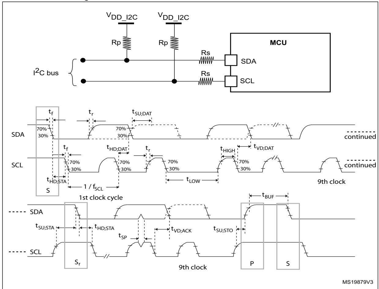
Figure 28. I 2 C bus AC waveforms and measurement circuit
