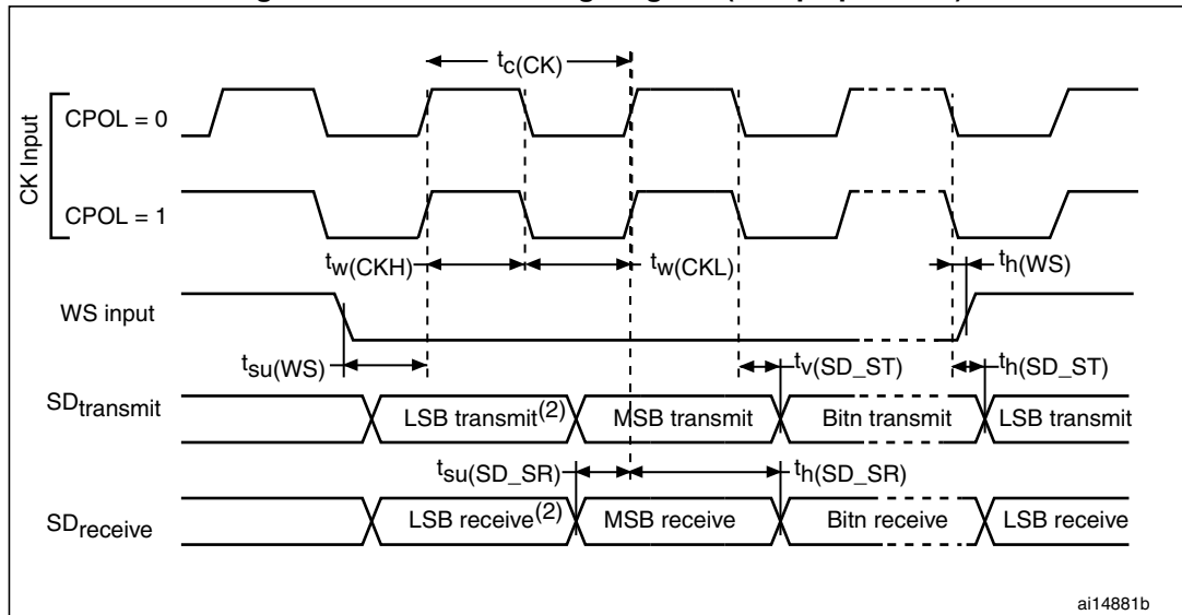
Figure 32. I2S slave timing diagram (Philips protocol)
