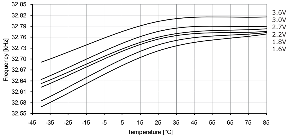
Figure 33-226. 32.768kHz internal oscillator frequency vs. temperature.
