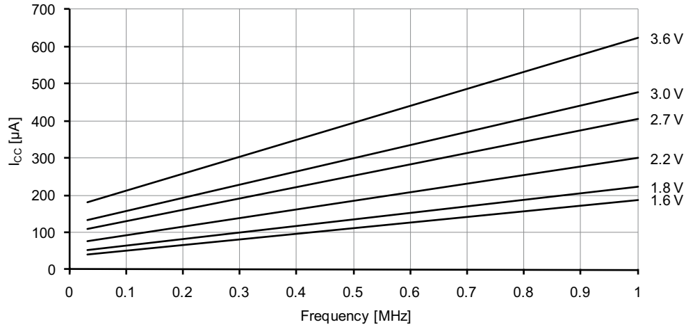
Figure 33-160. Active supply current vs. frequency.
