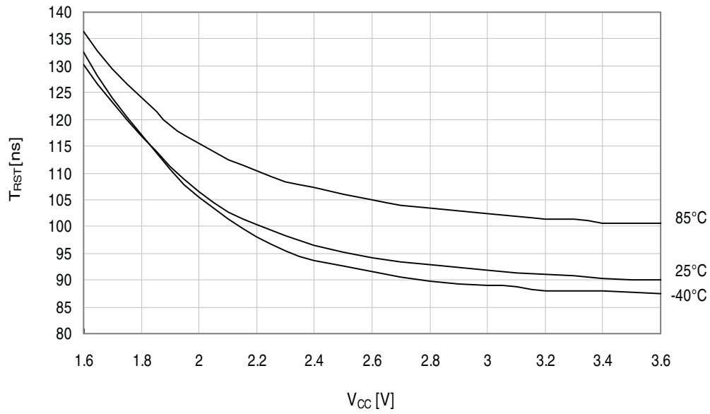
Figure 33-136. Minimum Reset pin pulse width vs. V_{CC} .
