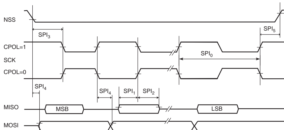
Figure 47-23.USART SPI Master Mode
