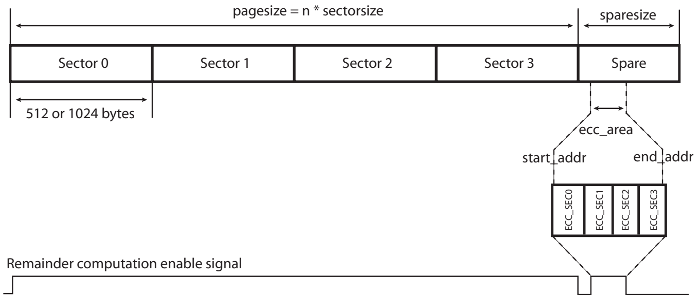
Figure 27-6. Read Operation
