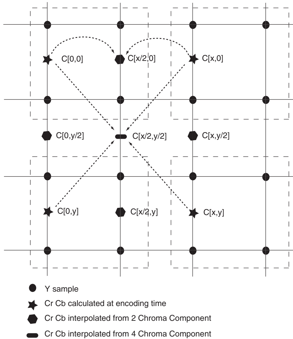
Figure 46-5. 4:2:0 Upsampling Algorithm
