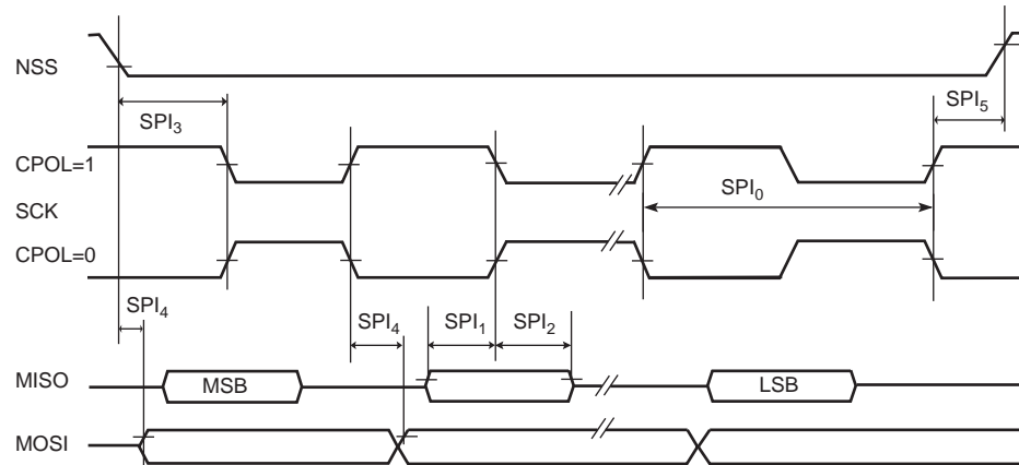
Figure 46-24. USART SPI Master Mode
