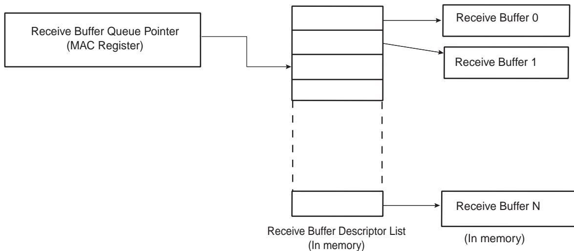
Figure 45-2. Receive Buffer List
