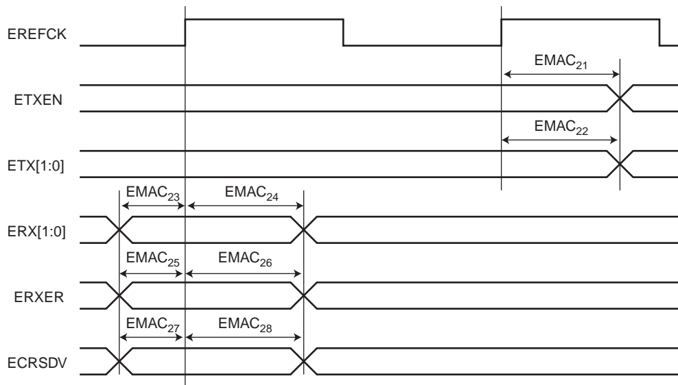
Figure 46-23. EMAC RMII Mode Signals
